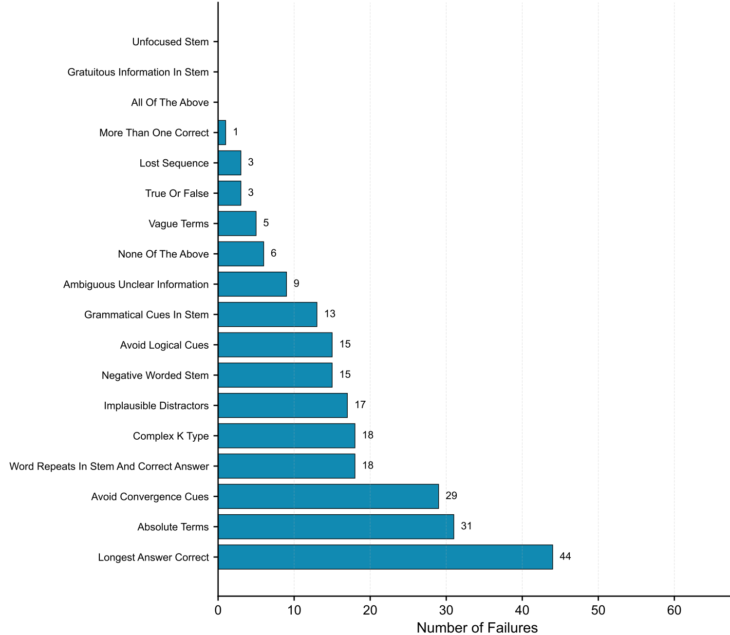
AI-Generated Questions (n=307)
