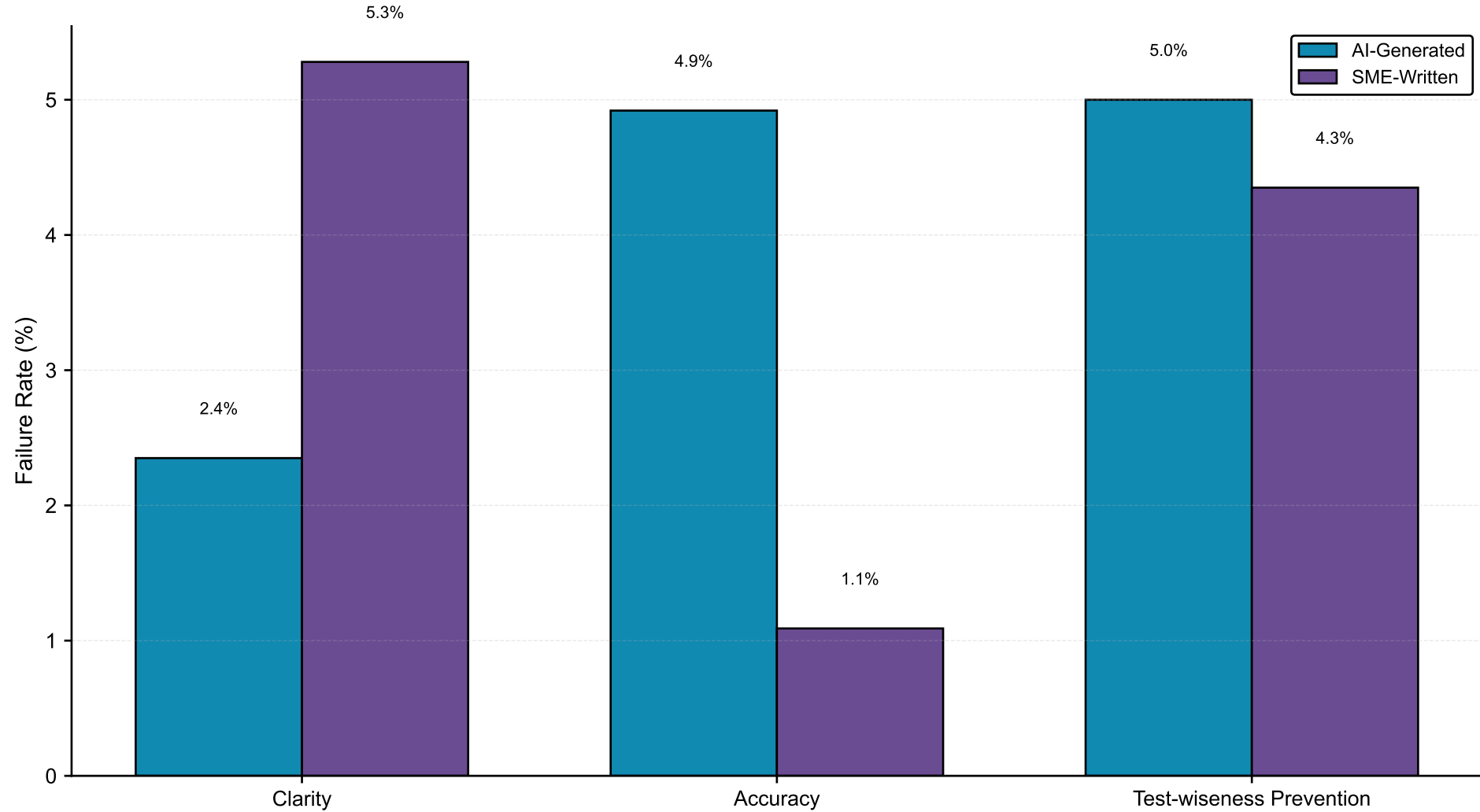
SAQUET Failure Rate by Category (AI-Generated vs SME-Written)
