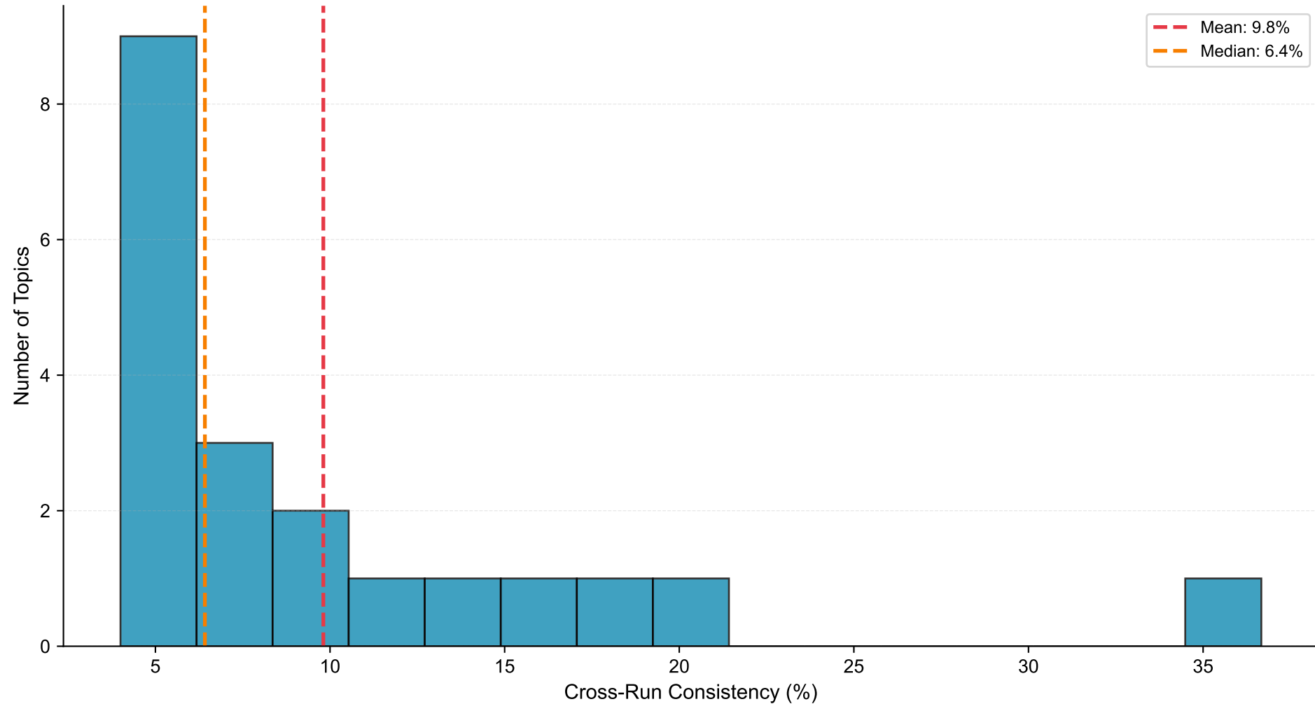
Distribution of Cross-Run Consistency Rates (Comparison across 4 runs, 10 questions each)
