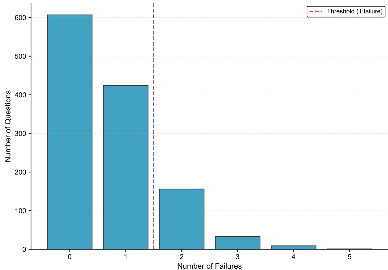
AI-Generated Questions: Failure Distribution
