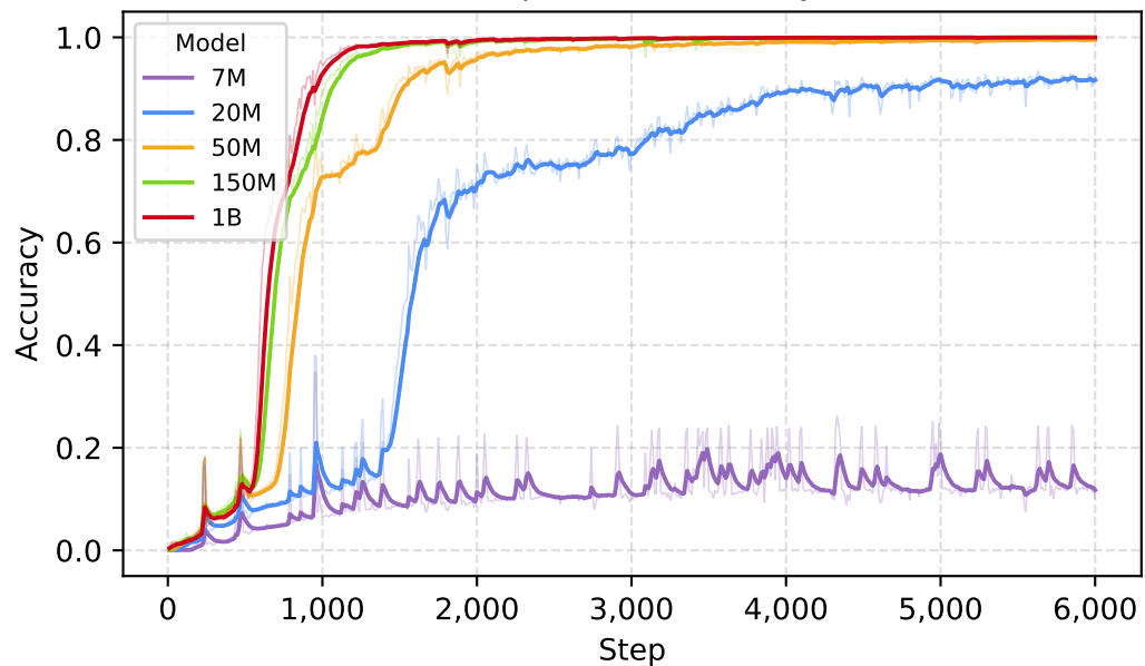
Decompression Accuracy
