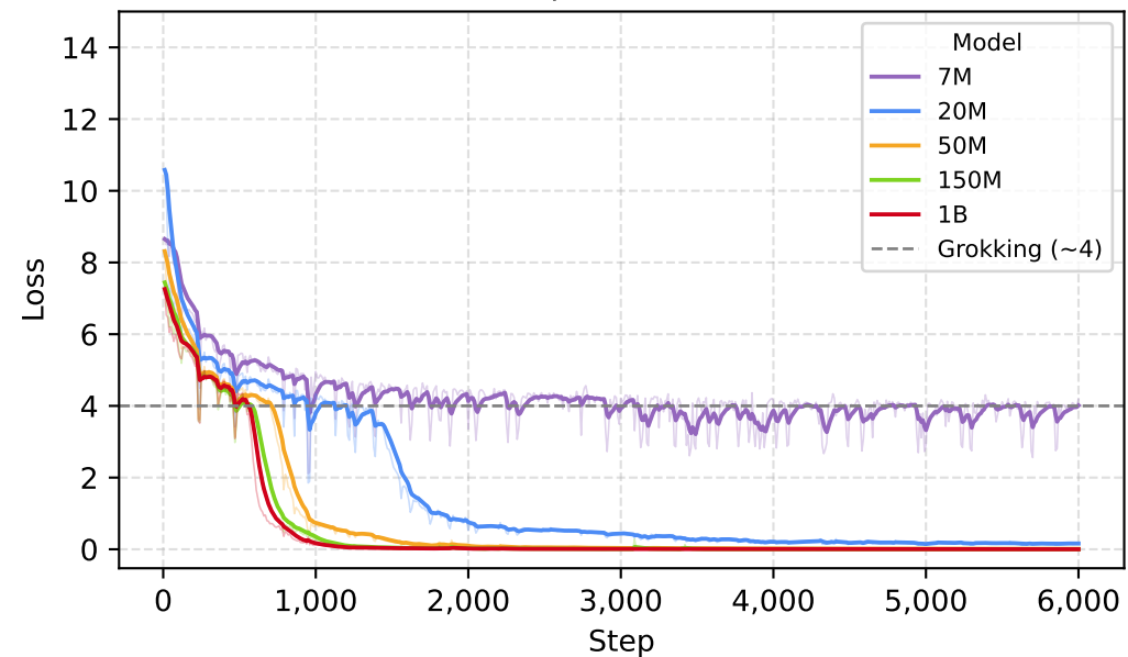
Decompression Loss
