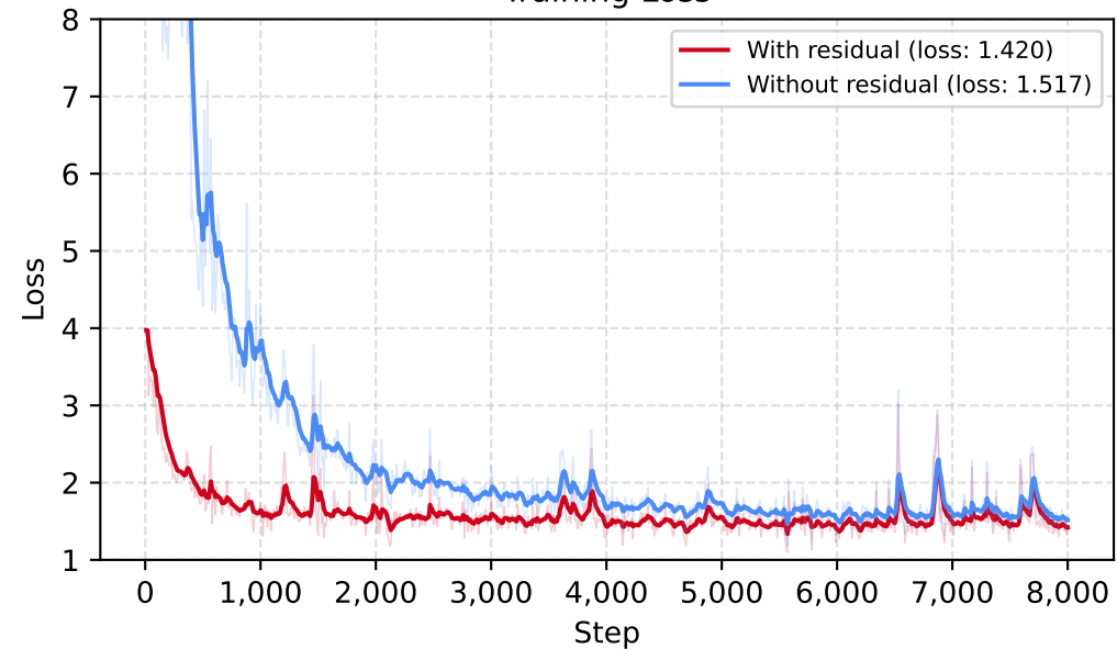
Training Loss
