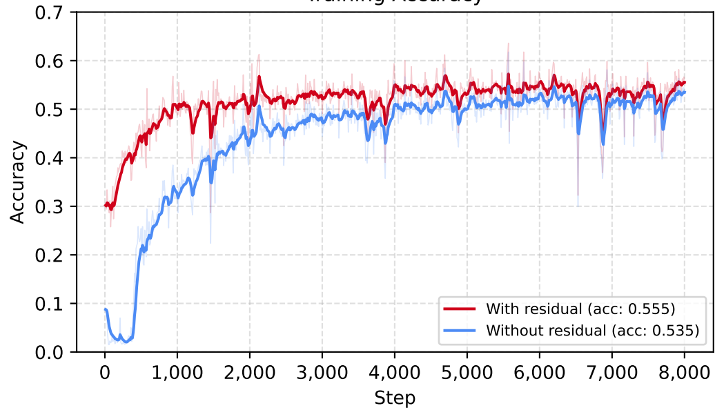
Training Accuracy
