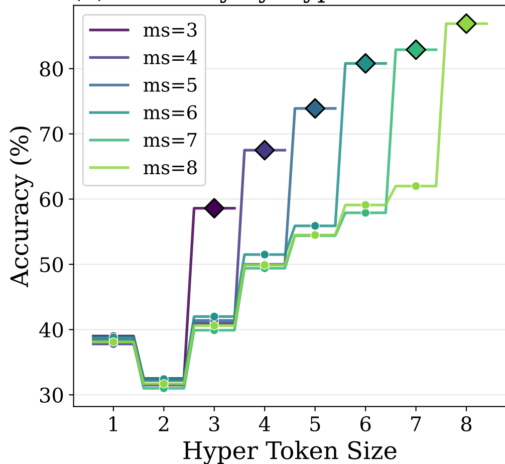
(a) Accuracy by Hyper Token Size
