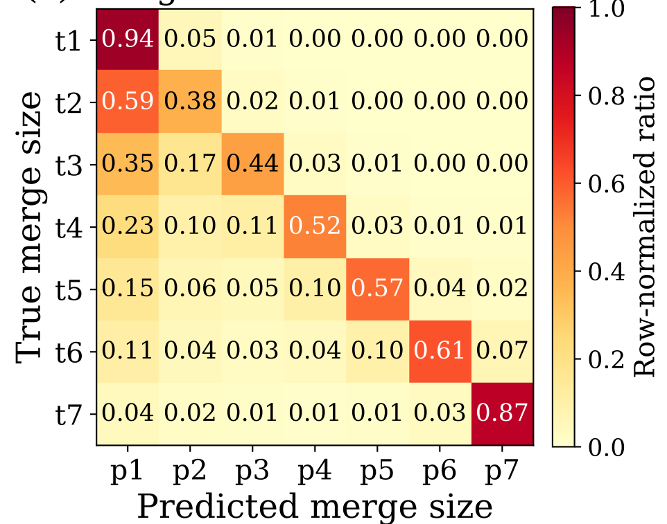
(c) Merge Size Confusion Matrix
