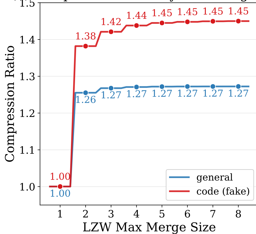
(b) Compression Ratio by Max Merge Size
