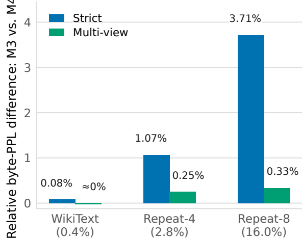
(b) Matched segmentation
