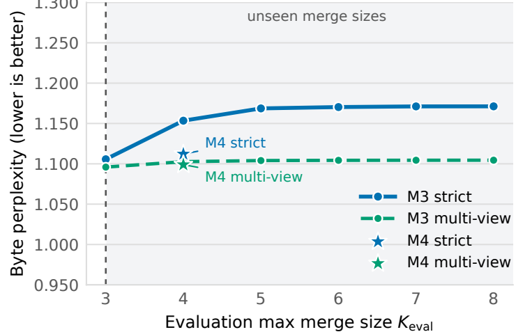
(c) Repeat-8 extrapolation
