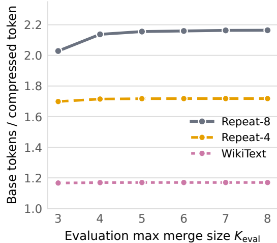
(a) Compression by corpus
