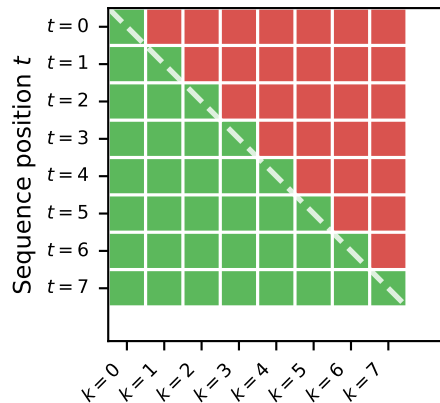
With hyper_causal_mask
