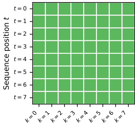
Without hyper_causal_mask
