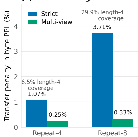
(c) Matched segmentation
