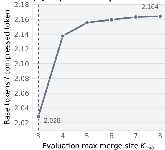
(b) Repeat-8 compression
