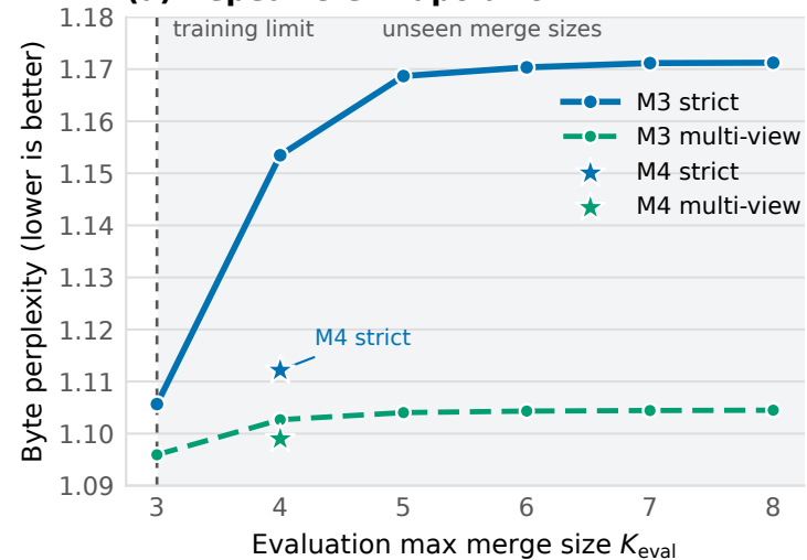
(a) Repeat-8 extrapolation
