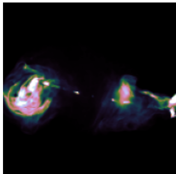
True image
