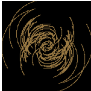
Sampling matrix
