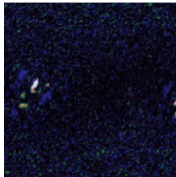
Dirty image
