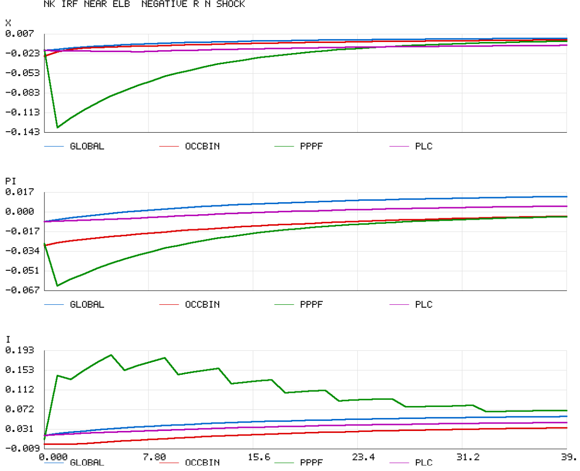
Figure 2: NK-ELB impulse responses (reference implementation): discretized global benchmark versus OccBin and PPPF-mixture approximations.
