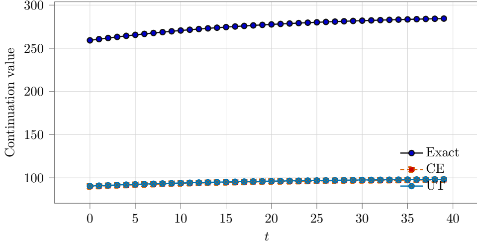
Figure 1: Burnside asset-pricing example: continuation-value response to a one-standard-deviation shock under the exact analytic benchmark, certainty equivalence (CE), and one-step sigma-point quadrature (UT).
