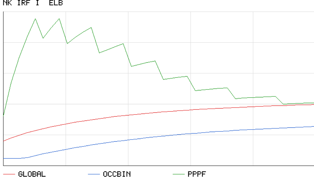
Figure 2: NK-ELB impulse responses (reference implementation): discretized global benchmark versus OccBin and PPPF-mixture approximations.
