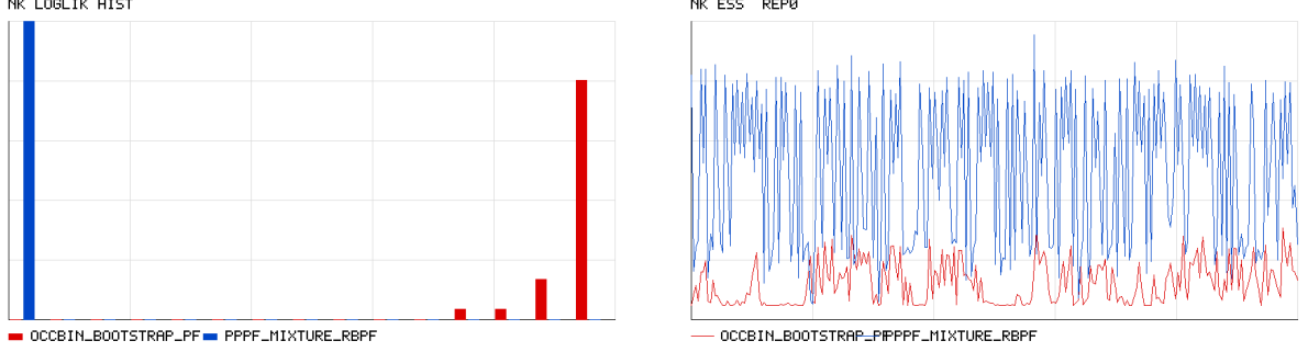
Figure 3: NK-ELB benchmark diagnostics (reference implementation): histogram of repeated log-likelihood estimates and ESS profile over time.
