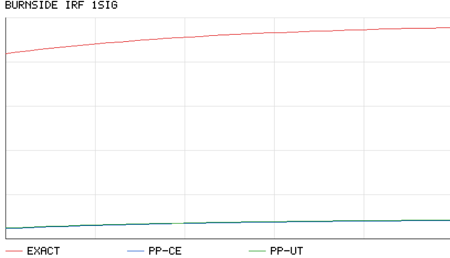
Figure 1: Burnside recursion validation (reference implementation): exact benchmark versus certainty equivalence (CE) and unscented-transform (UT) quadrature.
