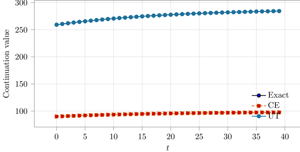
Figure 1: Burnside asset-pricing example: continuation-value response to a one-standard-deviation shock under the exact analytic benchmark, certainty equivalence (CE), and one-step positive-weight sigma-point quadrature (UT) with exact continuation.
