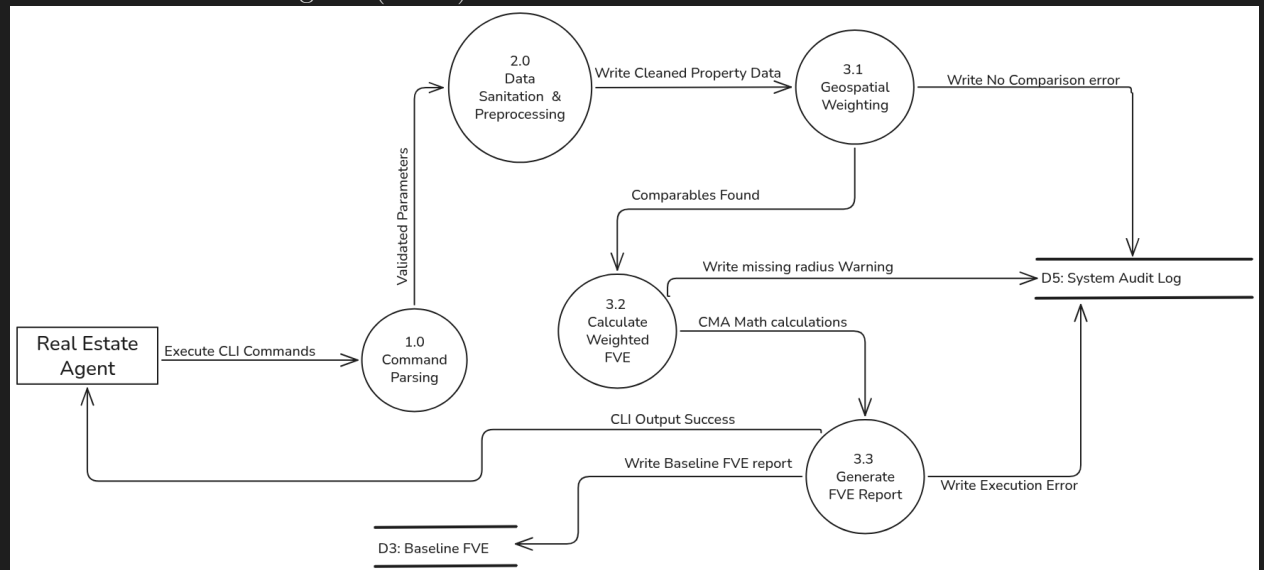
Level-2 Data Flow Diagram (2 of 3): Baseline FVE Process
