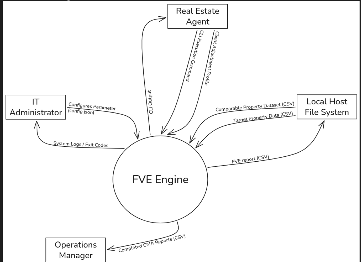
Shown are the various user classes and CSV file types, and how they interact. T Context-level Diagram
