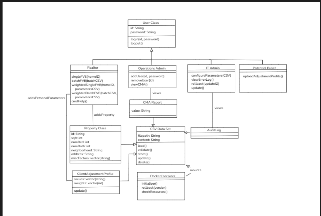
Shown are the various user classes and CSV file types, and how they interact. T Context-level Diagram
