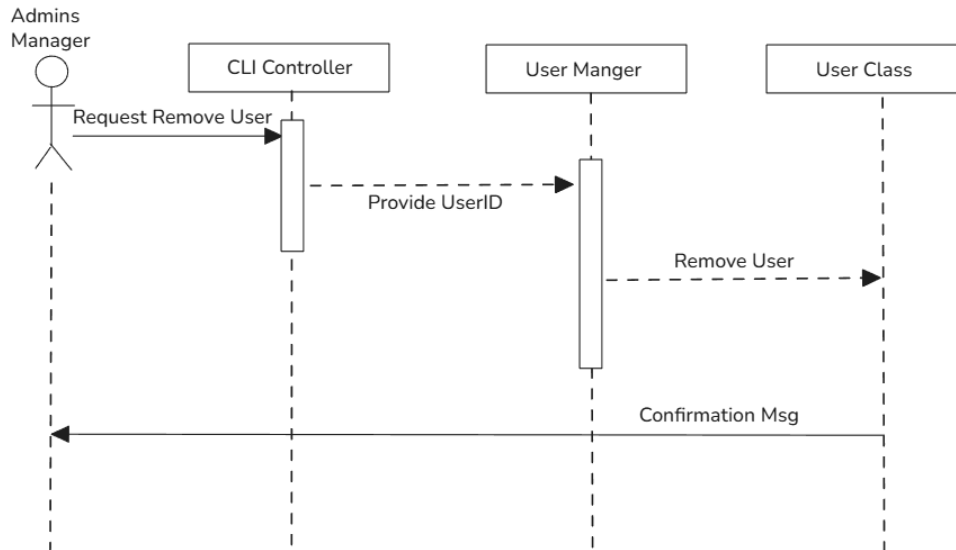
Sequence Diagram 7: Remove User
