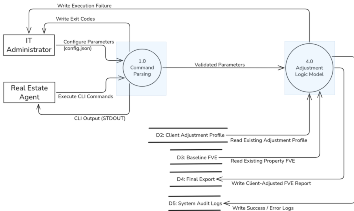
Level-1 Data Flow Diagram (2 of 2): Running Client Adjustment on preexisting properties with prior FVE
