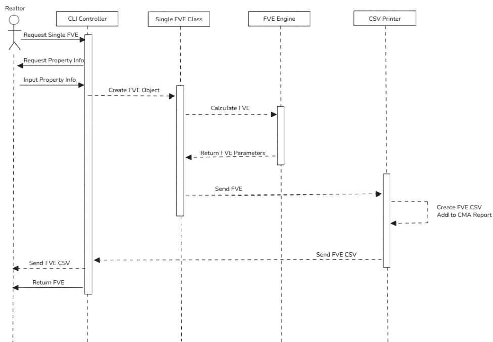
Sequence Diagram 1: Realtor Single FVE
