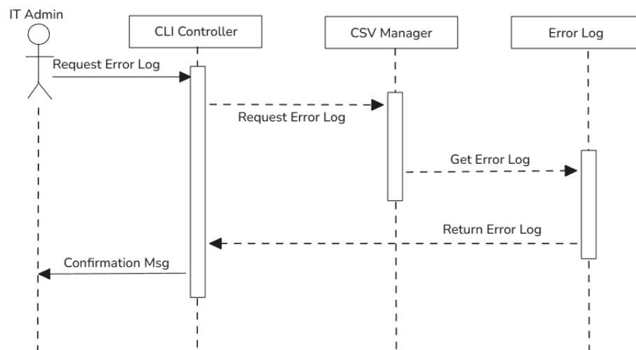
Sequence Diagram 8: View Error Log
