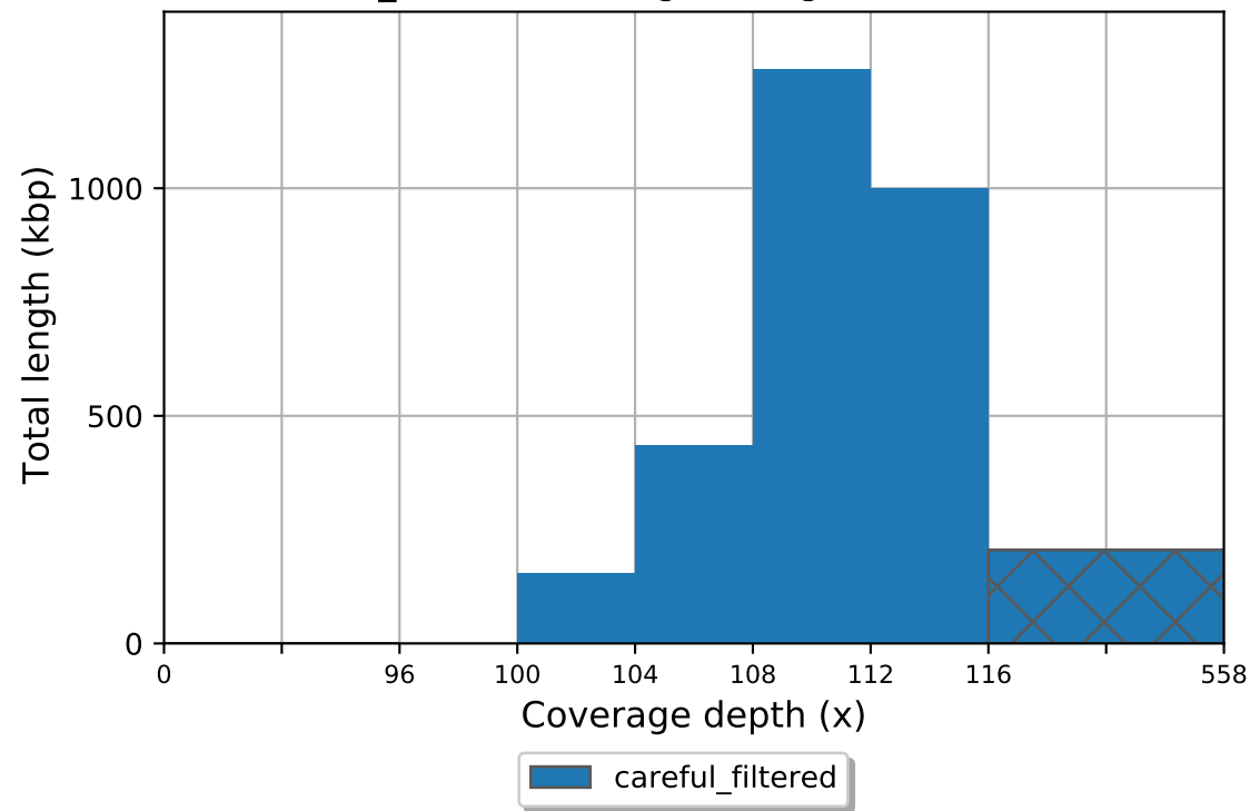
careful_filtered coverage histogram (bin size: 4x)
