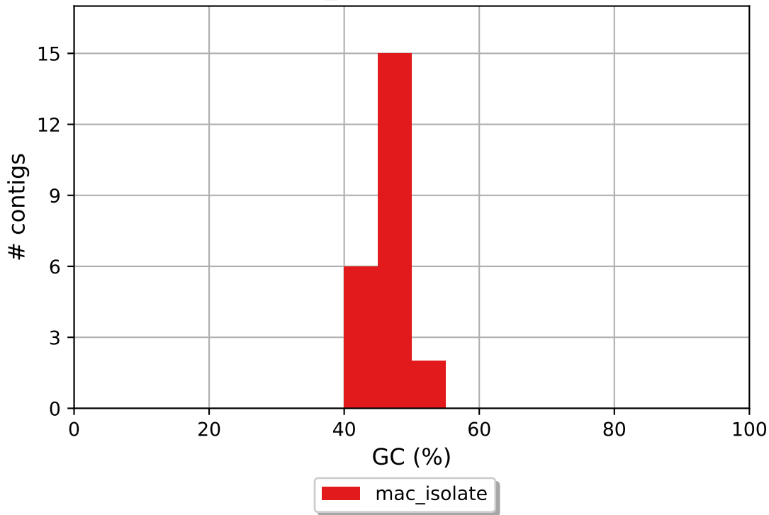
mac_isolate GC content
