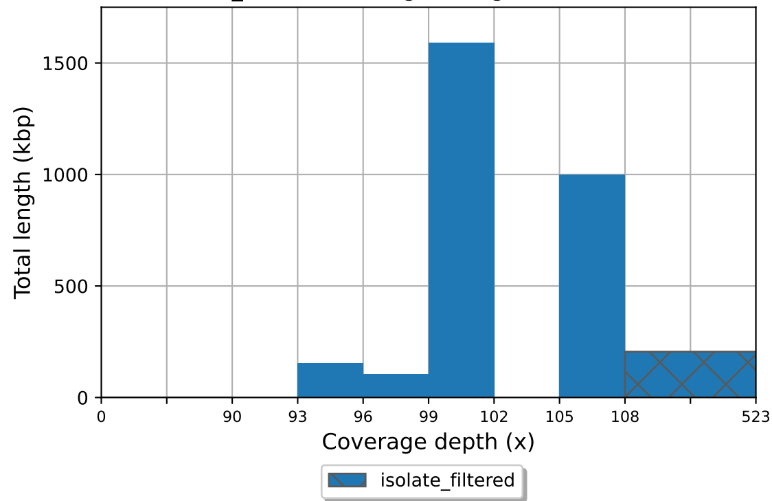
isolate_filtered coverage histogram (bin size: 3x)
