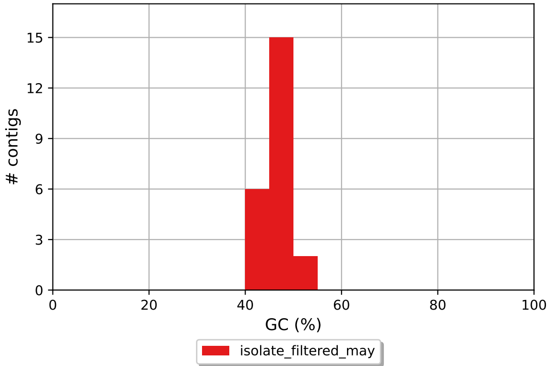
isolate_filtered_may GC content
