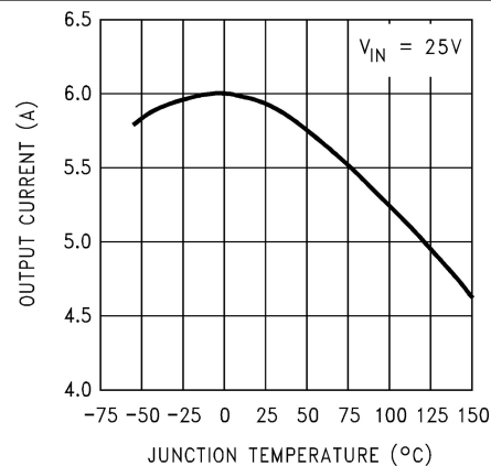
Figure 6-4. Current Limit
