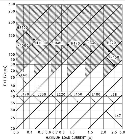
Figure 8-8. LM2576(HV)-ADJ
