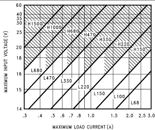
Figure 8-6. LM2576(HV)-12
