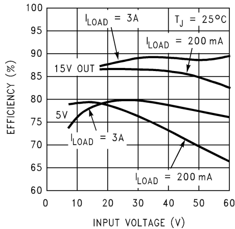
Figure 6-9. Efficiency
