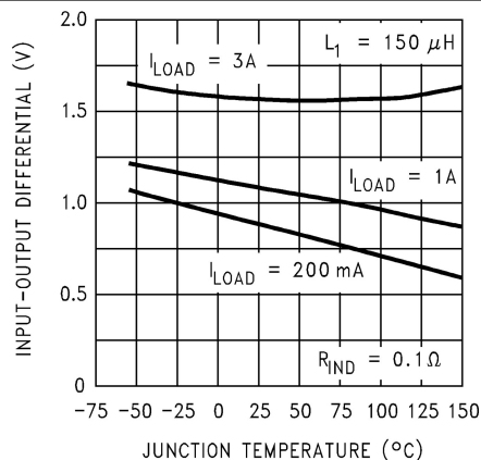
Figure 6-3. Dropout Voltage
