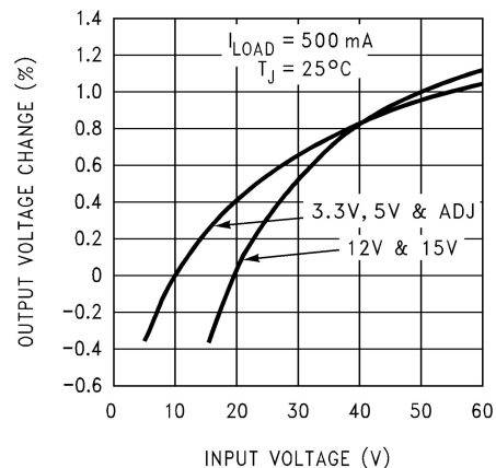
Figure 6-2. Line Regulation
