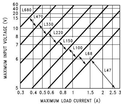
Figure 8-4. LM2576(HV)-3.3
