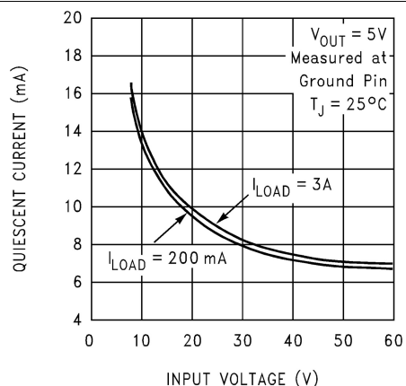
Figure 6-5. Quiescent Current
