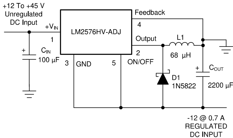
Figure 8-1. Inverting Buck-Boost Develops -12 V
