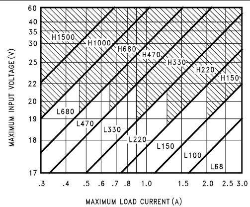
Figure 8-7. LM2576(HV)-15
