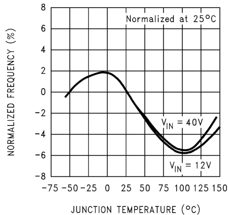
Figure 6-7. Oscillator Frequency
