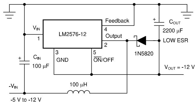
Figure 8-2. Negative Boost
