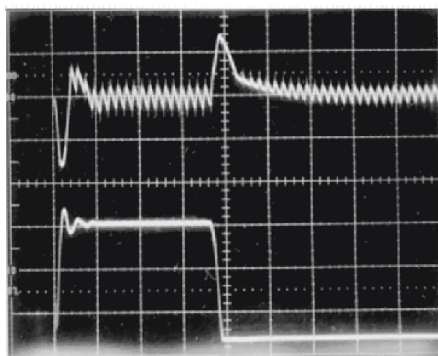
Figure 6-19. Load Transient Response
