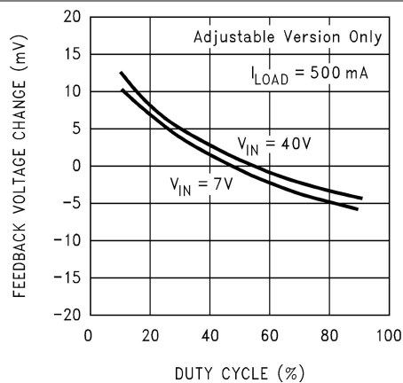
Figure 6-15. Feedback Voltage vs Duty Cycle
