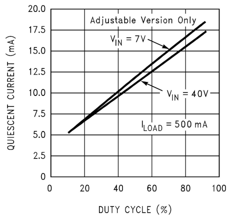
Figure 6-11. Quiescent Current vs Duty Cycle
