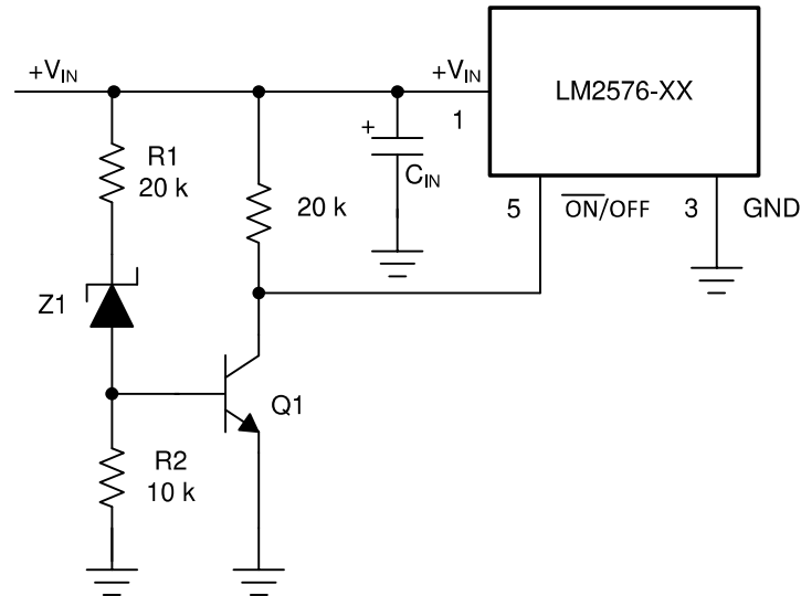
Figure 7-1. Undervoltage Lockout for Buck Circuit
