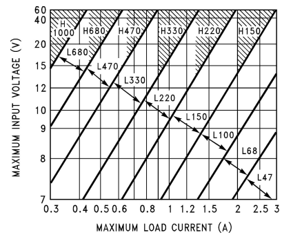
Figure 8-5. LM2576(HV)-5.0
