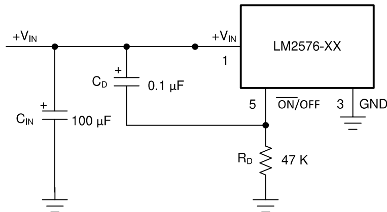
Figure 7-3. Delayed Start-Up
