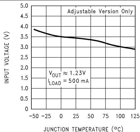
Figure 6-13. Minimum Operating Voltage
