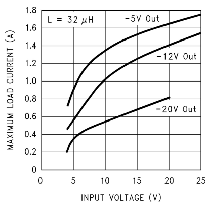
Figure 8-6. Inverting Regulator Typical Load Current
