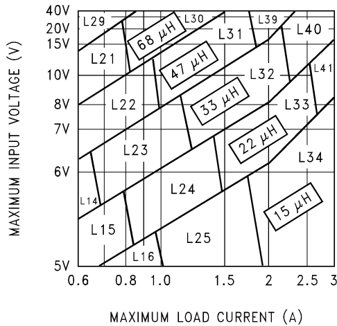
Figure 9-5. LM2596-3.3
