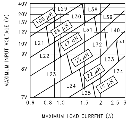
Figure 9-6. LM2596-5.0
