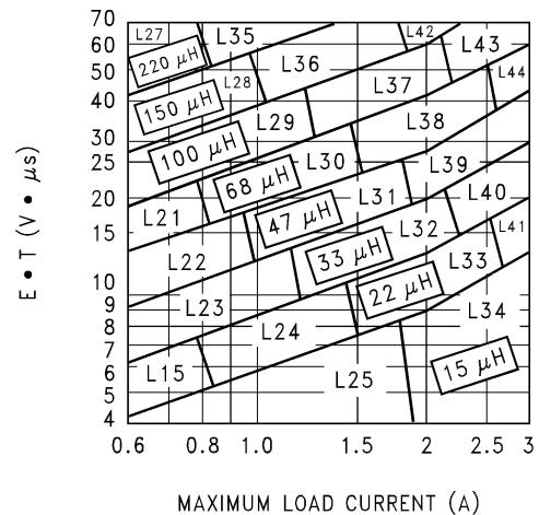
Figure 9-8. LM2596-ADJ
