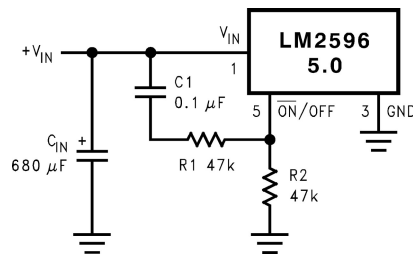
Figure 8-1. Delayed Start-Up
