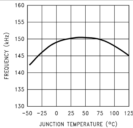
Figure 7-12. Switching Frequency
