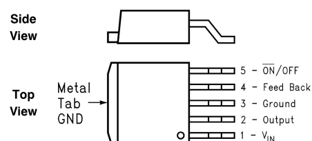
Figure 6-2. 5-Pin TO-263 KTT Package Top View
