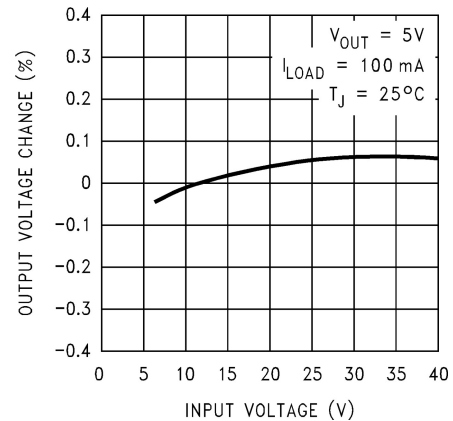
Figure 7-2. Line Regulation
