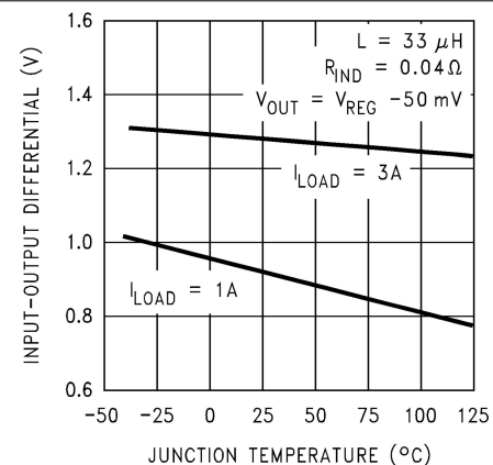
Figure 7-6. Dropout Voltage
