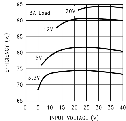
Figure 7-3. Efficiency
