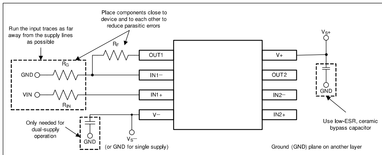
Figure 8-3. Operational Amplifier Board Layout for Noninverting Configuration
