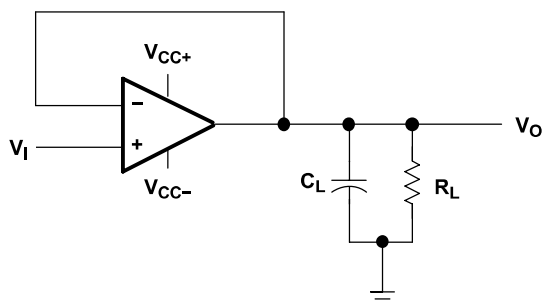
Figure 6-1. Unity-Gain Amplifier
