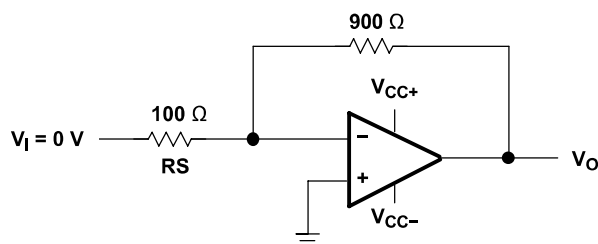
Figure 6-2. Noise-Test Circuit
