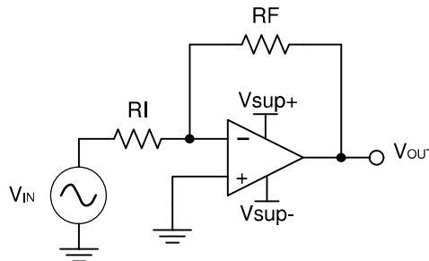
Figure 8-1. Application Schematic
