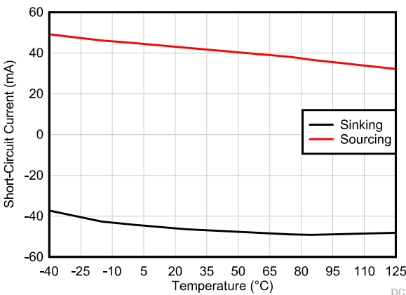
Figure 5-35. Short-Circuit Current vs Temperature
