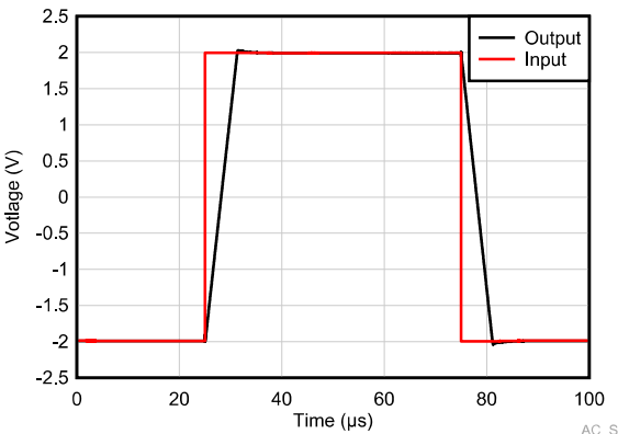
Figure 5-33. Large-Signal Step Response
