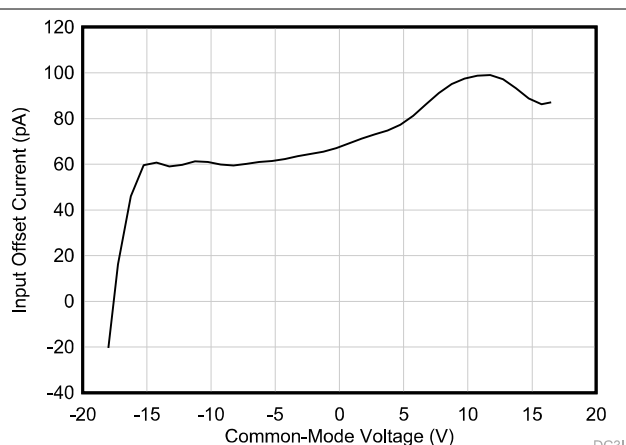
Figure 5-8. Input Offset Current vs Common-Mode Voltage
