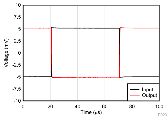
Figure 5-28. Overload Recovery
