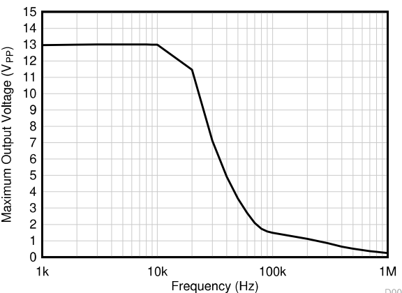
Figure 5-36. Maximum Output Voltage vs Frequency
