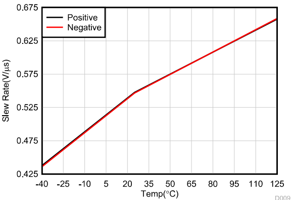
Figure 5-34. Slew Rate vs Temperature
