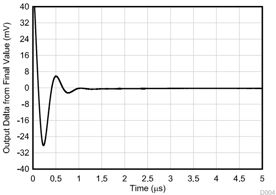
Figure 5-32. Large-Signal Step Response (Falling)
