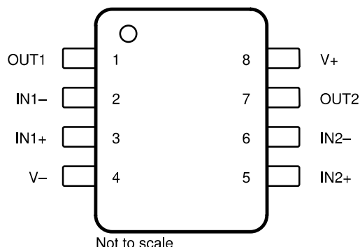
Figure 4-1. D, DDF, DGK, P, PS, PW, and JG Package 8-Pin SOIC, SOT23-8, VSSOP, PDIP, SO, TSSOP, and CDIP Top View
