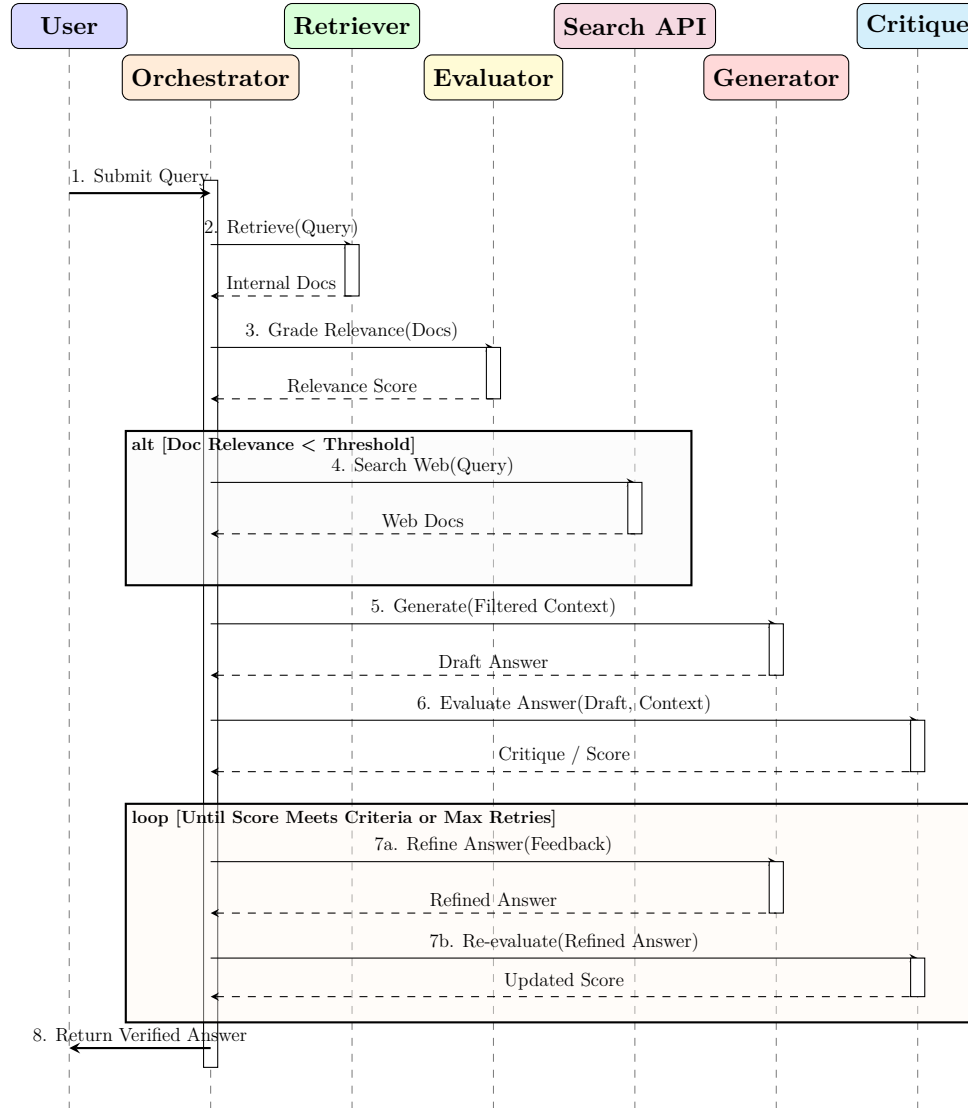
Figure 3: Self-Corrective RAG Sequence Diagram
