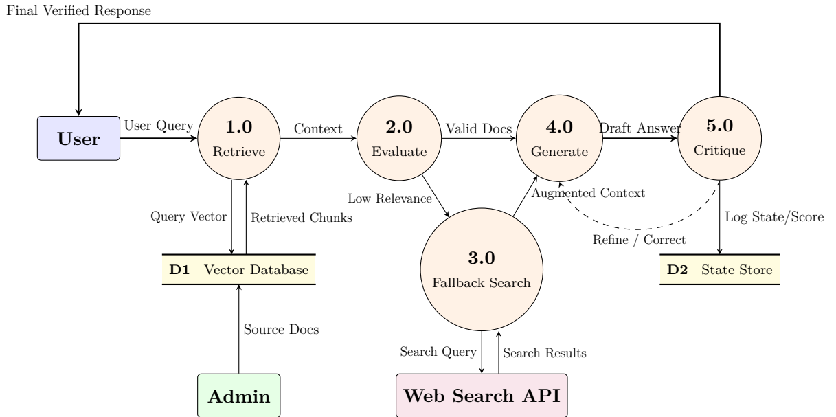
Figure 5: Level 1 Data Flow Diagram (DFD) for Self-Corrective RAG.
