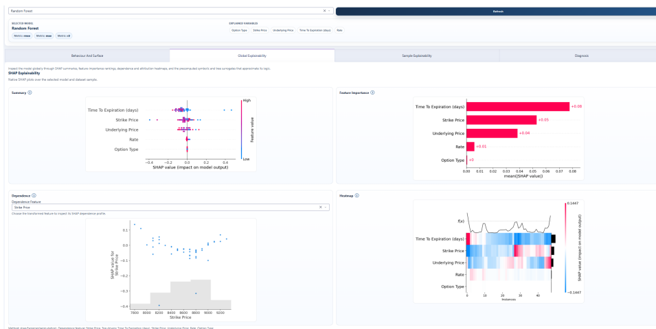
Figura 30: SHAP global Random Forest.
