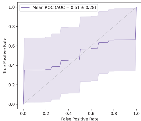
Cross Validation Patient Level (Before Batch Correction) Mean \pm SD ROC Curve
