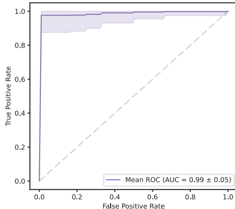
Cross Validation Patient Level (After Batch Correction) Mean \pm SD ROC Curve
