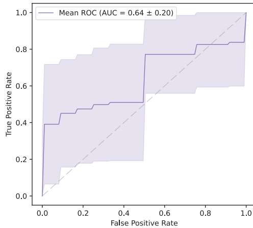
Institute Hold Out Patient Level (Before Batch Correction) Mean \pm SD ROC Curve
