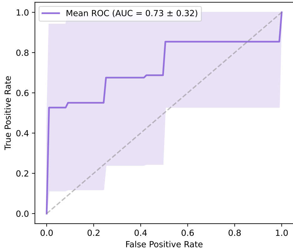
Institute Hold Out Patient Level (Keratinization and Telomeric Loci) Mean \pm SD ROC Curve
