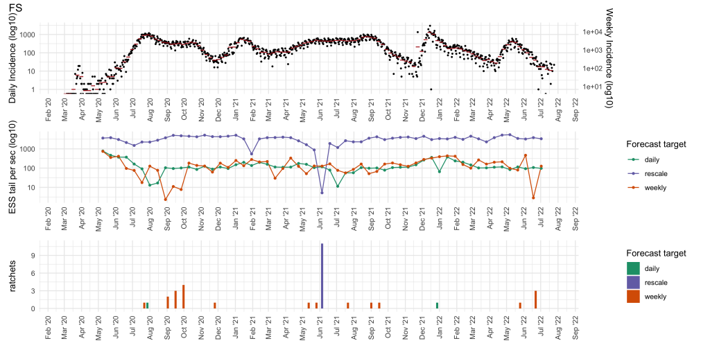
Figure 2. Computational diagnostics for the Free State province (FS). The top panel shows the daily and weekly COVID-19 incidence. The middle panel displays the tail Effective Sample Size (ESS) per second on a log10 scale, representing sampling efficiency for different forecast targets (colours). The bottom panel shows the number of model ratchets (adaptive refits) required to achieve convergence for each forecast slide.
