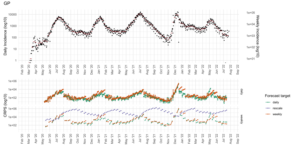
Figure 3. Forecast performance for the Gauteng province (GP). The top panel shows the daily (black points) and weekly (red horizontal segments) COVID-19 incidence. The bottom panel displays the Continuous Ranked Probability Score (CRPS) for daily, weekly, and rescaled weekly forecast targets (colours), with both incidence and CRPS shown on a log10 scale. The rows in the bottom panel are faceted by the temporal resolution of the evaluation data (daily or weekly).
