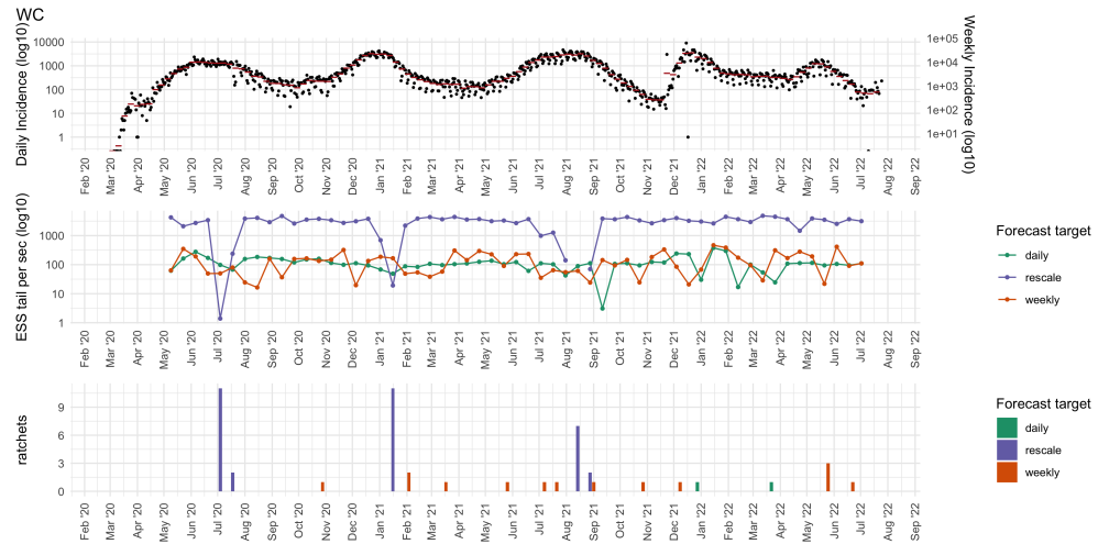
Figure 16. Computational diagnostics for the Western Cape province (WC). The top panel shows the daily and weekly COVID-19 incidence. The middle panel displays the tail Effective Sample Size (ESS) per second on a log10 scale, representing sampling efficiency for different forecast targets (colours). The bottom panel shows the number of model ratchets (adaptive refits) required to achieve convergence for each forecast slide.
