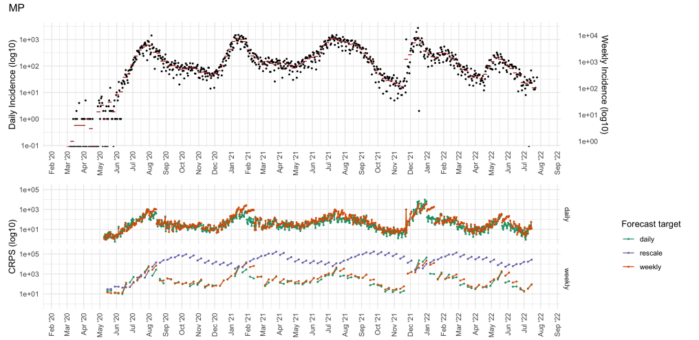
Figure 9. Forecast performance for the Mpumalanga province (MP). The top panel shows the daily (black points) and weekly (red horizontal segments) COVID-19 incidence. The bottom panel displays the Continuous Ranked Probability Score (CRPS) for daily, weekly, and rescaled weekly forecast targets (colours), with both incidence and CRPS shown on a log10 scale. The rows in the bottom panel are faceted by the temporal resolution of the evaluation data (daily or weekly).
