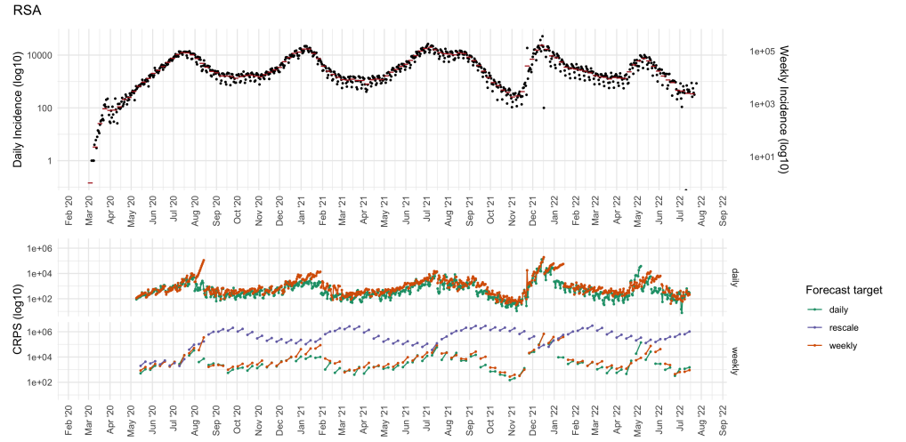
Figure 17. Forecast performance for the national aggregate (RSA). The top panel shows the daily (black points) and weekly (red horizontal segments) COVID-19 incidence. The bottom panel displays the Continuous Ranked Probability Score (CRPS) for daily, weekly, and rescaled weekly forecast targets (colours), with both incidence and CRPS shown on a log10 scale. The rows in the bottom panel are faceted by the temporal resolution of the evaluation data (daily or weekly).
