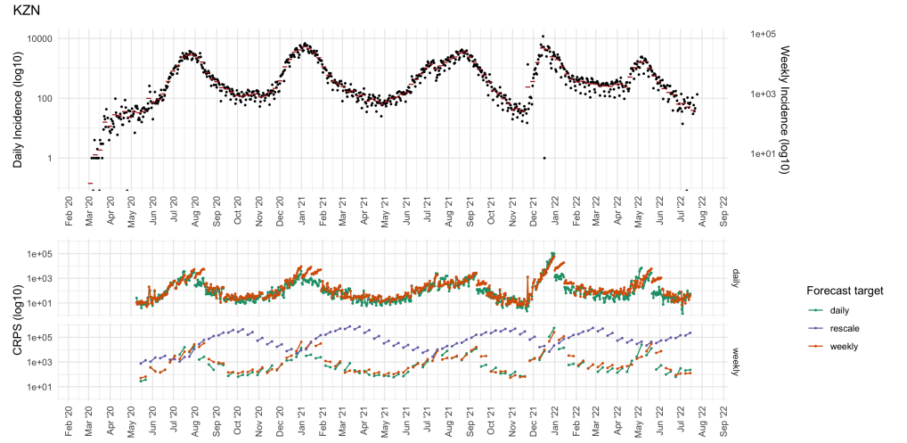
Figure 5. Forecast performance for the KwaZulu-Natal province (KZN). The top panel shows the daily (black points) and weekly (red horizontal segments) COVID-19 incidence. The bottom panel displays the Continuous Ranked Probability Score (CRPS) for daily, weekly, and rescaled weekly forecast targets (colours), with both incidence and CRPS shown on a log10 scale. The rows in the bottom panel are faceted by the temporal resolution of the evaluation data (daily or weekly).
