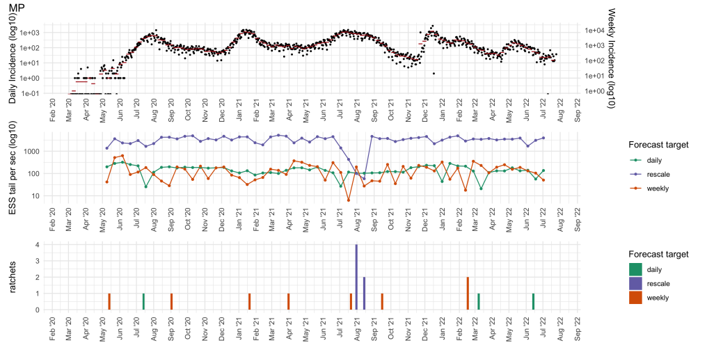
Figure 10. Computational diagnostics for the Mpumalanga province (MP). The top panel shows the daily and weekly COVID-19 incidence. The middle panel displays the tail Effective Sample Size (ESS) per second on a log10 scale, representing sampling efficiency for different forecast targets (colours). The bottom panel shows the number of model ratchets (adaptive refits) required to achieve convergence for each forecast slide.
