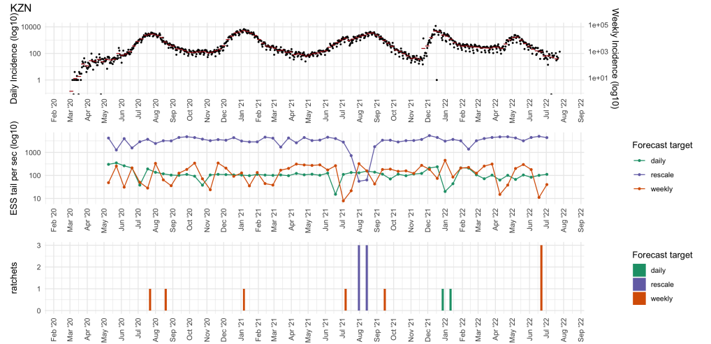
Figure 6. Computational diagnostics for the KwaZulu-Natal province (KZN). The top panel shows the daily and weekly COVID-19 incidence. The middle panel displays the tail Effective Sample Size (ESS) per second on a log10 scale, representing sampling efficiency for different forecast targets (colours). The bottom panel shows the number of model ratchets (adaptive refits) required to achieve convergence for each forecast slide.
