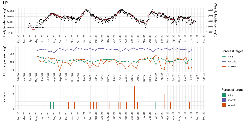
Figure 8. Computational diagnostics for the Limpopo province (LP). The top panel shows the daily and weekly COVID-19 incidence. The middle panel displays the tail Effective Sample Size (ESS) per second on a log10 scale, representing sampling efficiency for different forecast targets (colours). The bottom panel shows the number of model ratchets (adaptive refits) required to achieve convergence for each forecast slide.
