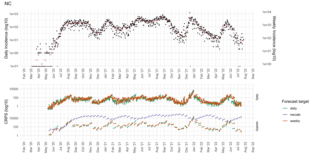
Figure 11. Forecast performance for the Northern Cape province (NC). The top panel shows the daily (black points) and weekly (red horizontal segments) COVID-19 incidence. The bottom panel displays the Continuous Ranked Probability Score (CRPS) for daily, weekly, and rescaled weekly forecast targets (colours), with both incidence and CRPS shown on a log10 scale. The rows in the bottom panel are faceted by the temporal resolution of the evaluation data (daily or weekly).
