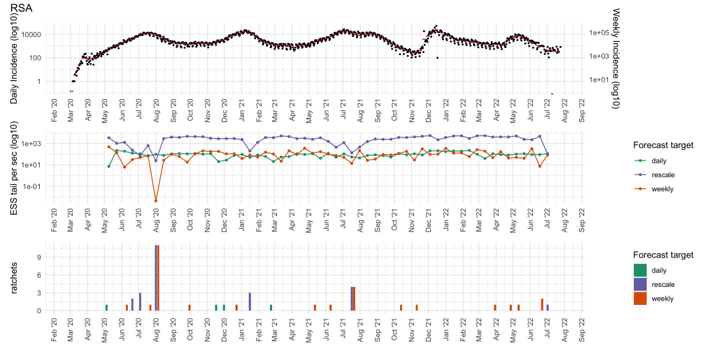
Figure 18. Computational diagnostics for the national aggregate (RSA). The top panel shows the daily and weekly COVID-19 incidence. The middle panel displays the tail Effective Sample Size (ESS) per second on a log10 scale, representing sampling efficiency for different forecast targets (colours). The bottom panel shows the number of model ratchets (adaptive refits) required to achieve convergence for each forecast slide.
