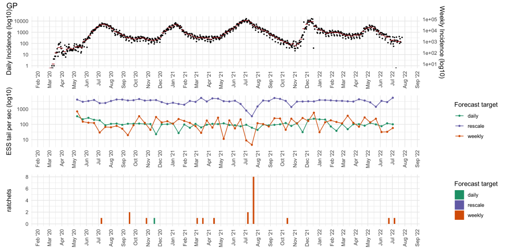
Figure 4. Computational diagnostics for the Gauteng province (GP). The top panel shows the daily and weekly COVID-19 incidence. The middle panel displays the tail Effective Sample Size (ESS) per second on a log10 scale, representing sampling efficiency for different forecast targets (colours). The bottom panel shows the number of model ratchets (adaptive refits) required to achieve convergence for each forecast slide.
