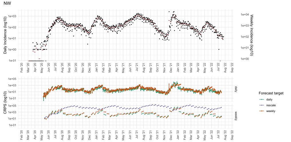
Figure 13. Forecast performance for the North West province (NW). The top panel shows the daily (black points) and weekly (red horizontal segments) COVID-19 incidence. The bottom panel displays the Continuous Ranked Probability Score (CRPS) for daily, weekly, and rescaled weekly forecast targets (colours), with both incidence and CRPS shown on a log10 scale. The rows in the bottom panel are faceted by the temporal resolution of the evaluation data (daily or weekly).
