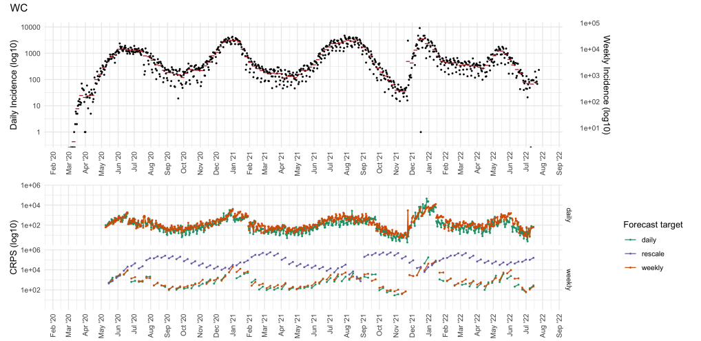
Figure 15. Forecast performance for the Western Cape province (WC). The top panel shows the daily (black points) and weekly (red horizontal segments) COVID-19 incidence. The bottom panel displays the Continuous Ranked Probability Score (CRPS) for daily, weekly, and rescaled weekly forecast targets (colours), with both incidence and CRPS shown on a log10 scale. The rows in the bottom panel are faceted by the temporal resolution of the evaluation data (daily or weekly).
