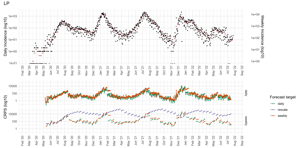
Figure 7. Forecast performance for the Limpopo province (LP). The top panel shows the daily (black points) and weekly (red horizontal segments) COVID-19 incidence. The bottom panel displays the Continuous Ranked Probability Score (CRPS) for daily, weekly, and rescaled weekly forecast targets (colours), with both incidence and CRPS shown on a log10 scale. The rows in the bottom panel are faceted by the temporal resolution of the evaluation data (daily or weekly).
