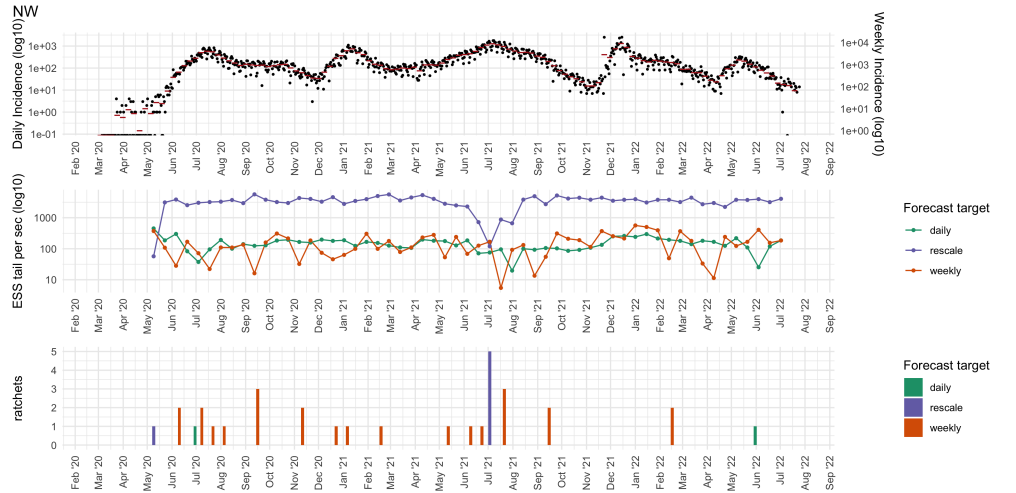
Figure 14. Computational diagnostics for the North West province (NW). The top panel shows the daily and weekly COVID-19 incidence. The middle panel displays the tail Effective Sample Size (ESS) per second on a log10 scale, representing sampling efficiency for different forecast targets (colours). The bottom panel shows the number of model ratchets (adaptive refits) required to achieve convergence for each forecast slide.
