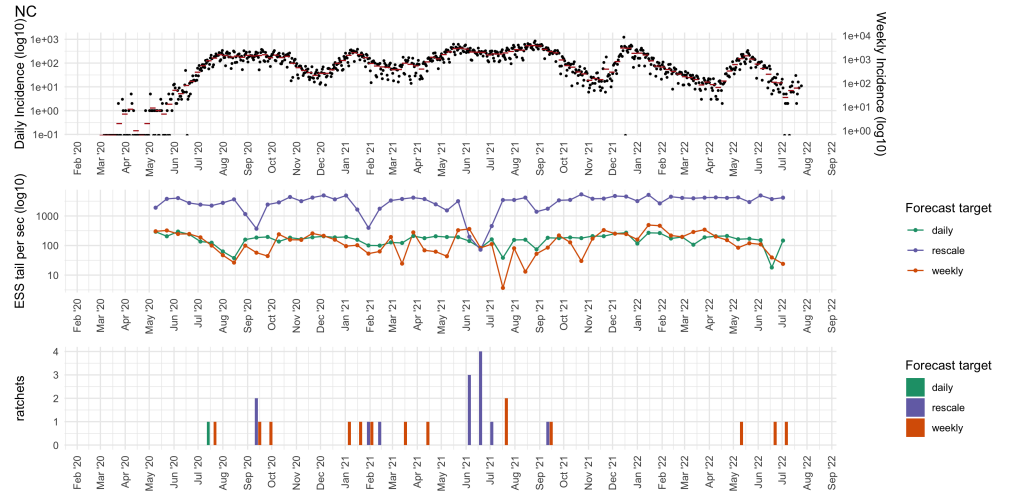
Figure 12. Computational diagnostics for the Northern Cape province (NC). The top panel shows the daily and weekly COVID-19 incidence. The middle panel displays the tail Effective Sample Size (ESS) per second on a log10 scale, representing sampling efficiency for different forecast targets (colours). The bottom panel shows the number of model ratchets (adaptive refits) required to achieve convergence for each forecast slide.
