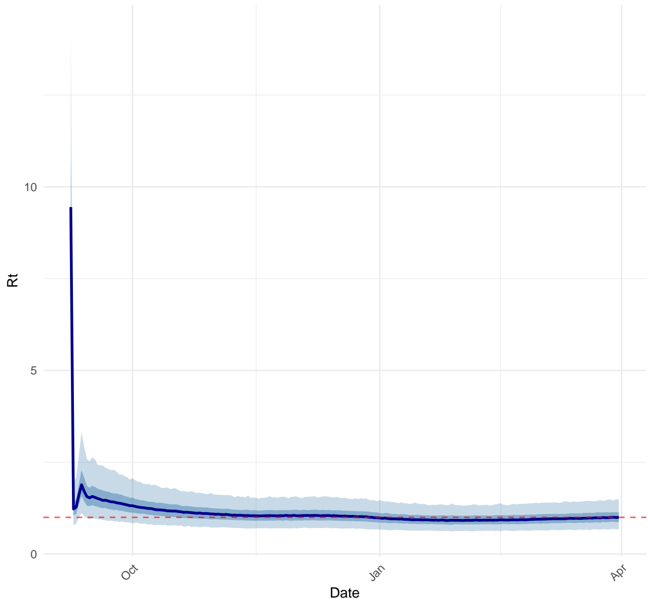
Estimated Reproduction Number ( R_t ) Over Time Ribbon shows 50% (dark) and 95% (light) credible intervals
