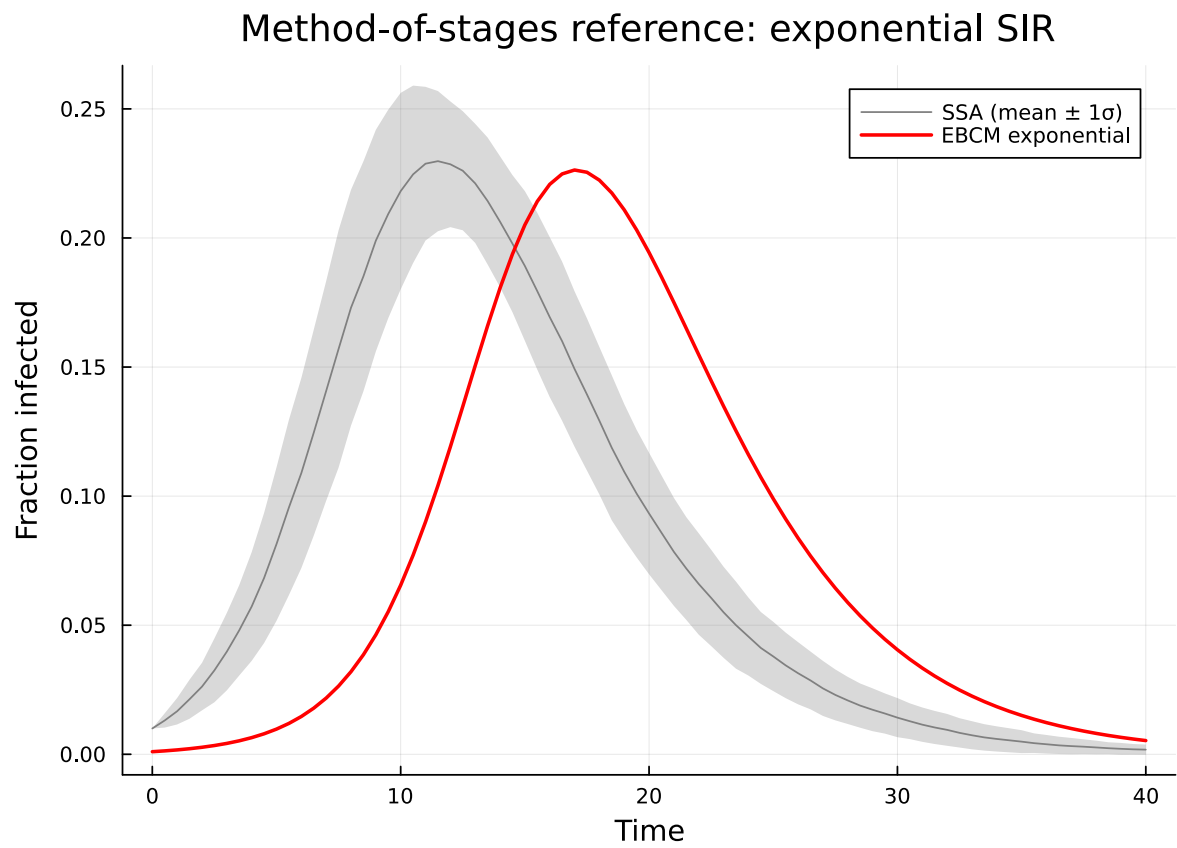
Figure 6: Figure 6: Exponential EBCM (red line) vs Gillespie SSA mean \pm 1\sigma (gray).
