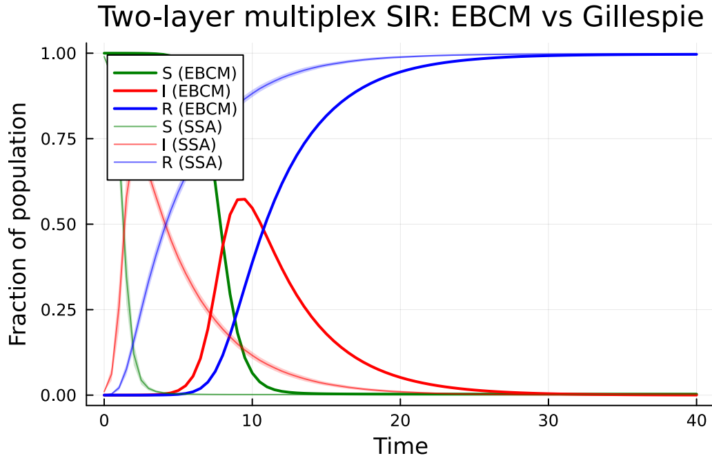
Figure 10: Two-layer multiplex EBCM (lines) vs Gillespie SSA on a MultiplexNetwork host graph (mean \pm 1\sigma ribbons across 5 graphs \times 20 sims). Layer weights \beta_{11}=0.75 , \beta_{22}=0.25 ; layers are Poisson(3) and Poisson(8) on N=1000 .
