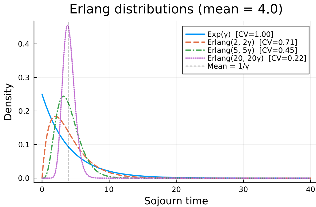
Figure 1: Erlang distributions with the same mean ( 1/\gamma = 4 ) but increasing shape parameter n . As n increases, the distribution concentrates around the mean.
