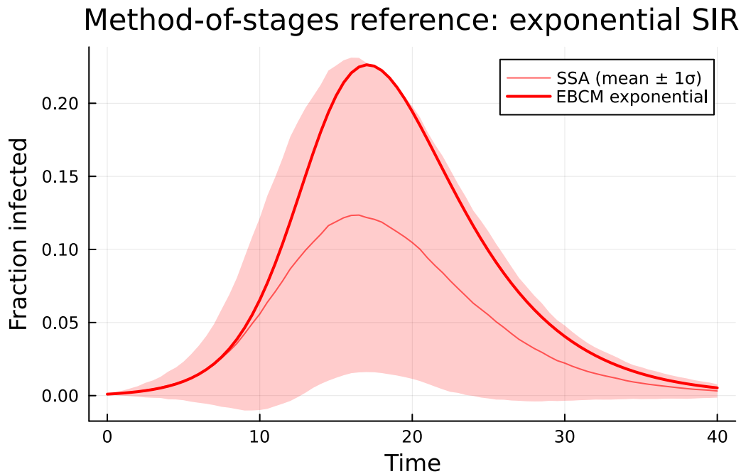
Figure 6: Exponential EBCM (red line) vs Gillespie SSA mean \pm 1\sigma (red ribbon).
