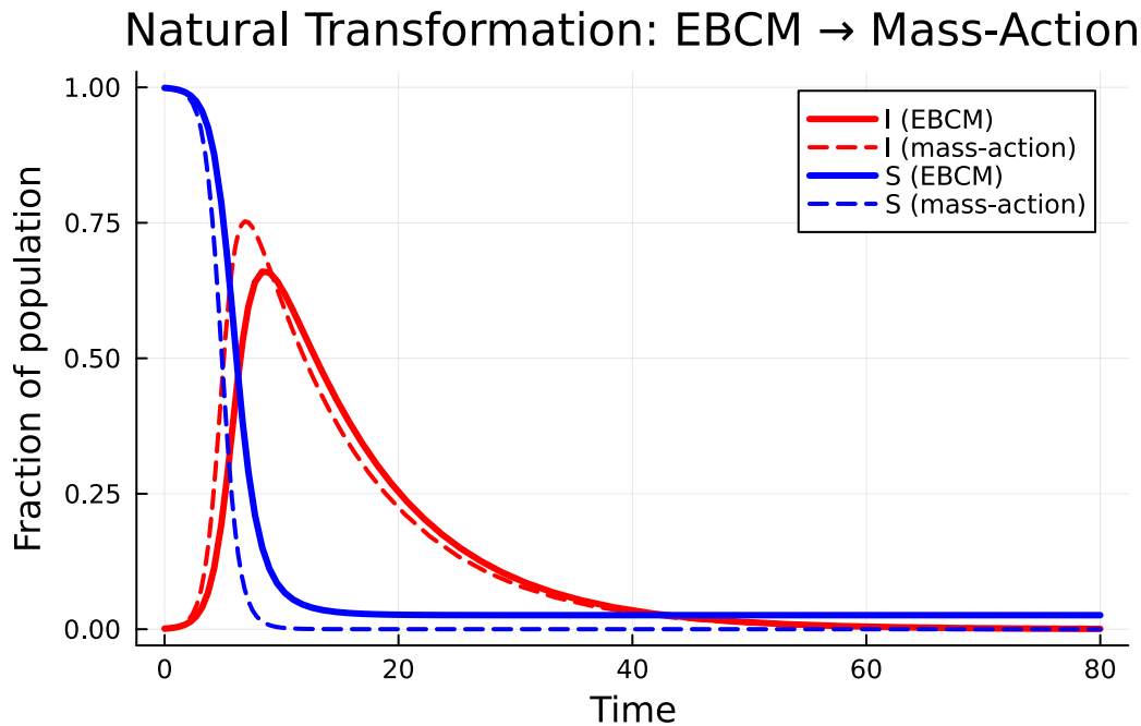
Figure 3: EBCM vs mass-action approximation on a Poisson(5) network.
