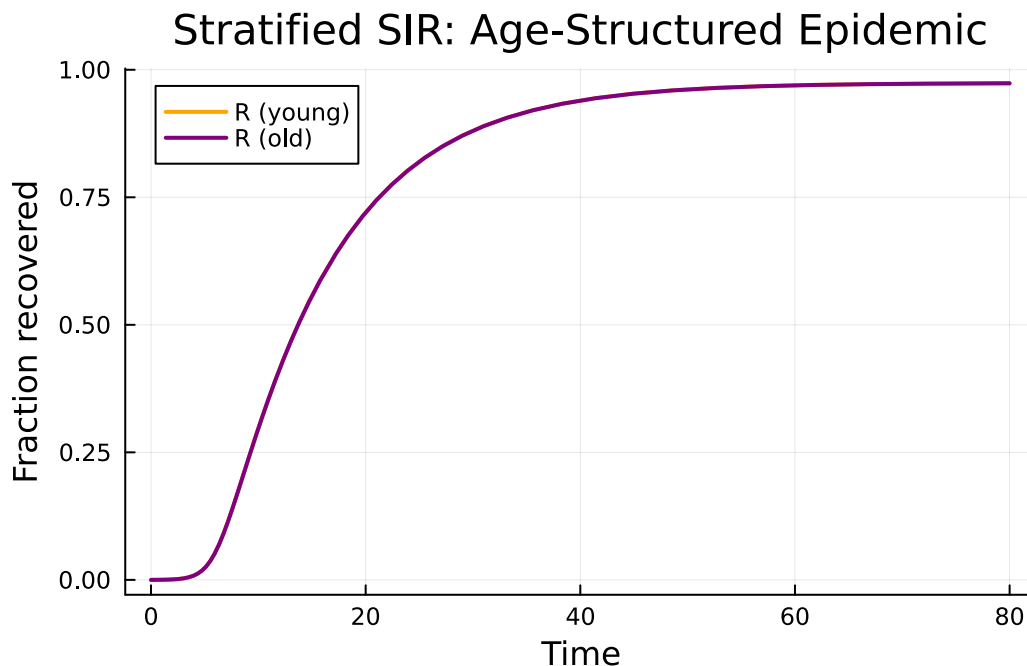
Figure 2: Stratified SIR: young and old populations with assortative contact mixing.
