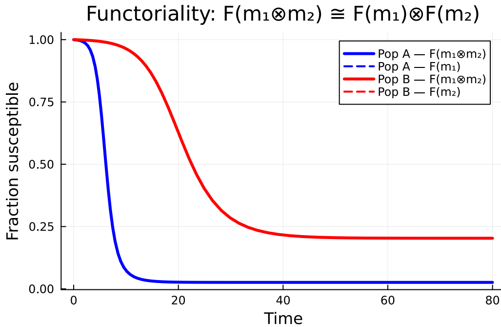
Figure 4: Functoriality check: F(m_1 \otimes m_2) matches F(m_1), F(m_2) to machine precision.
