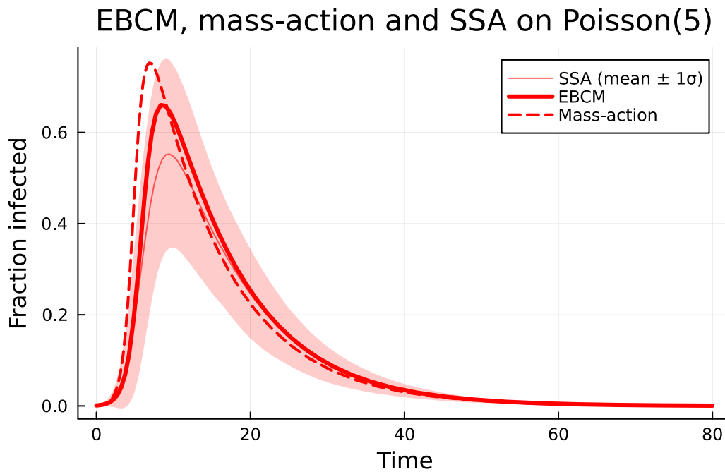
Figure 5: EBCM (red) and mass-action approximation (red dashed) versus Gillespie SSA mean \pm 1\sigma (red ribbon).
