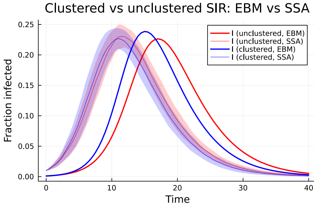
Figure 5: EBM (lines) versus DirectSSA (ribbons = mean \pm 1\sigma across 36 trajectories on 3 graphs of N=2000 ). Both networks have mean degree 5; the clustered network is built via the Newman–Miller doubly Poisson construction with \kappa_s=3 , \kappa_t=1 .
