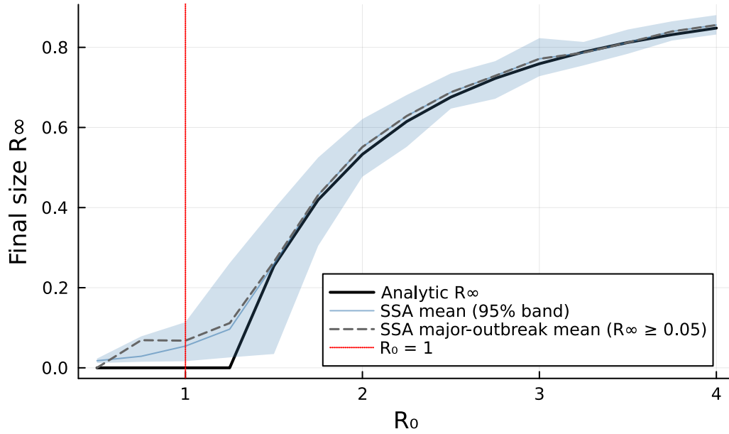
Figure 6: Analytic final size (line) versus DirectSSA on Erdős–Rényi graphs ( N=2000 , ribbon = 95% empirical interval across 36 trajectories per R_0 ). Major / minor outbreak bimodality near the threshold widens the band; subset-conditioned curve overlaid in grey.
