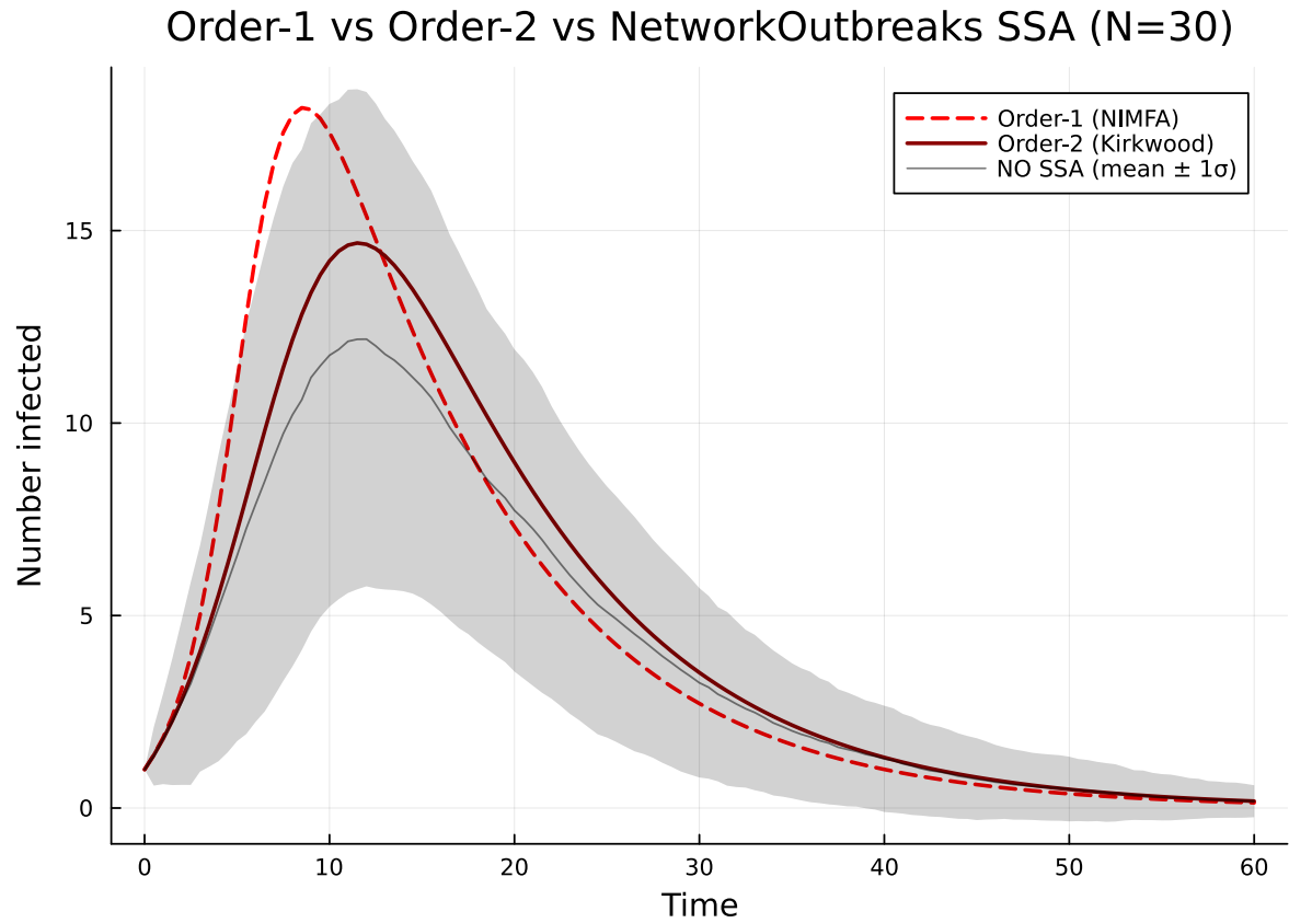
Figure 1: NetworkOutbreaks SSA mean \pm 1\sigma ribbon (12 host graphs \times 25 SSA replicates) overlaid on order-1 (NIMFA) and order-2 (Kirkwood) deterministic trajectories. The exact stochastic distribution sits between (and slightly below) both deterministic closures, consistent with the documented closure ordering.
