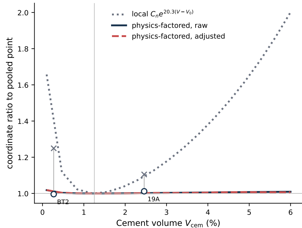
Local exponential versus factored coordinate
