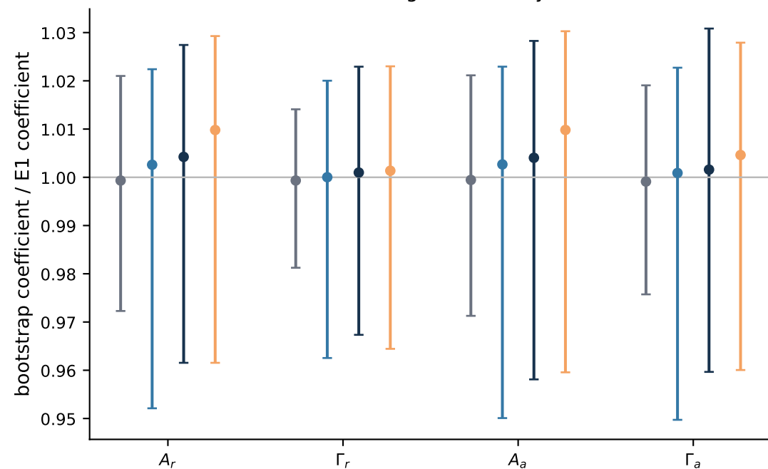
Block-length sensitivity
