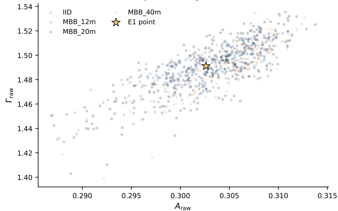
Block-length sensitivity
