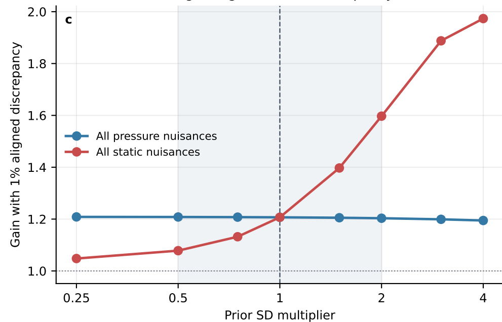
Target-aligned model discrepancy
