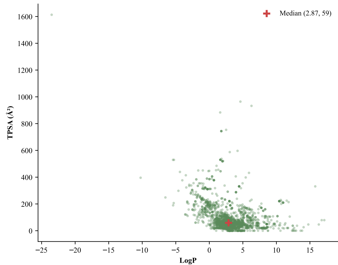
D. LogP × TPSA chemical-property envelope
