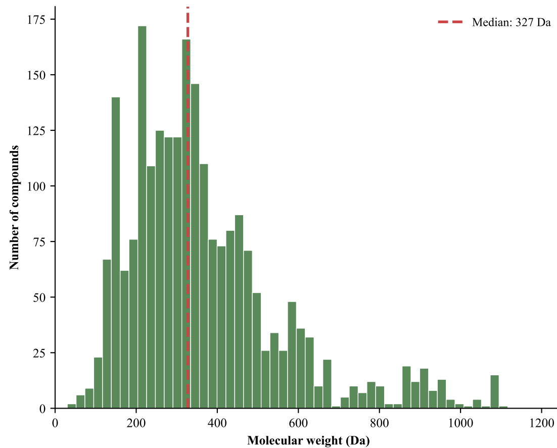
C. Molecular weight distribution (n=17 outliers >1200 Da hidden)
