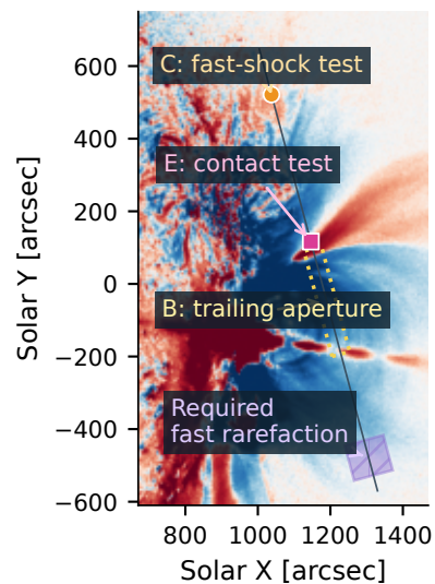
(b) Same frame minus 15:30:24 UT
