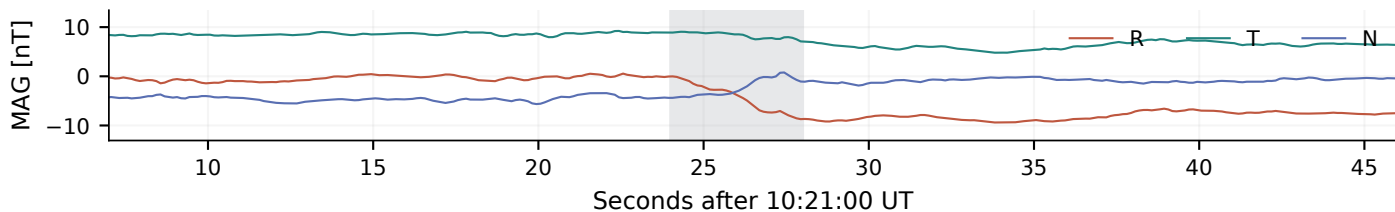
(e) Solar Orbiter | 30 August 2021 | boundary core shaded
