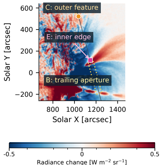
(e) Solar Orbiter | 30 August 2021 | boundary core shaded
