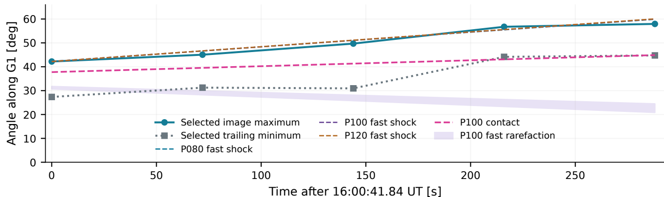
(d) First maximum aligned once; later model positions predicted
