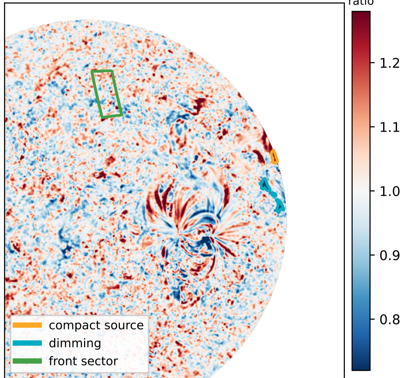
(a) Fixed regions in AIA 171 Å late/pre ratio
