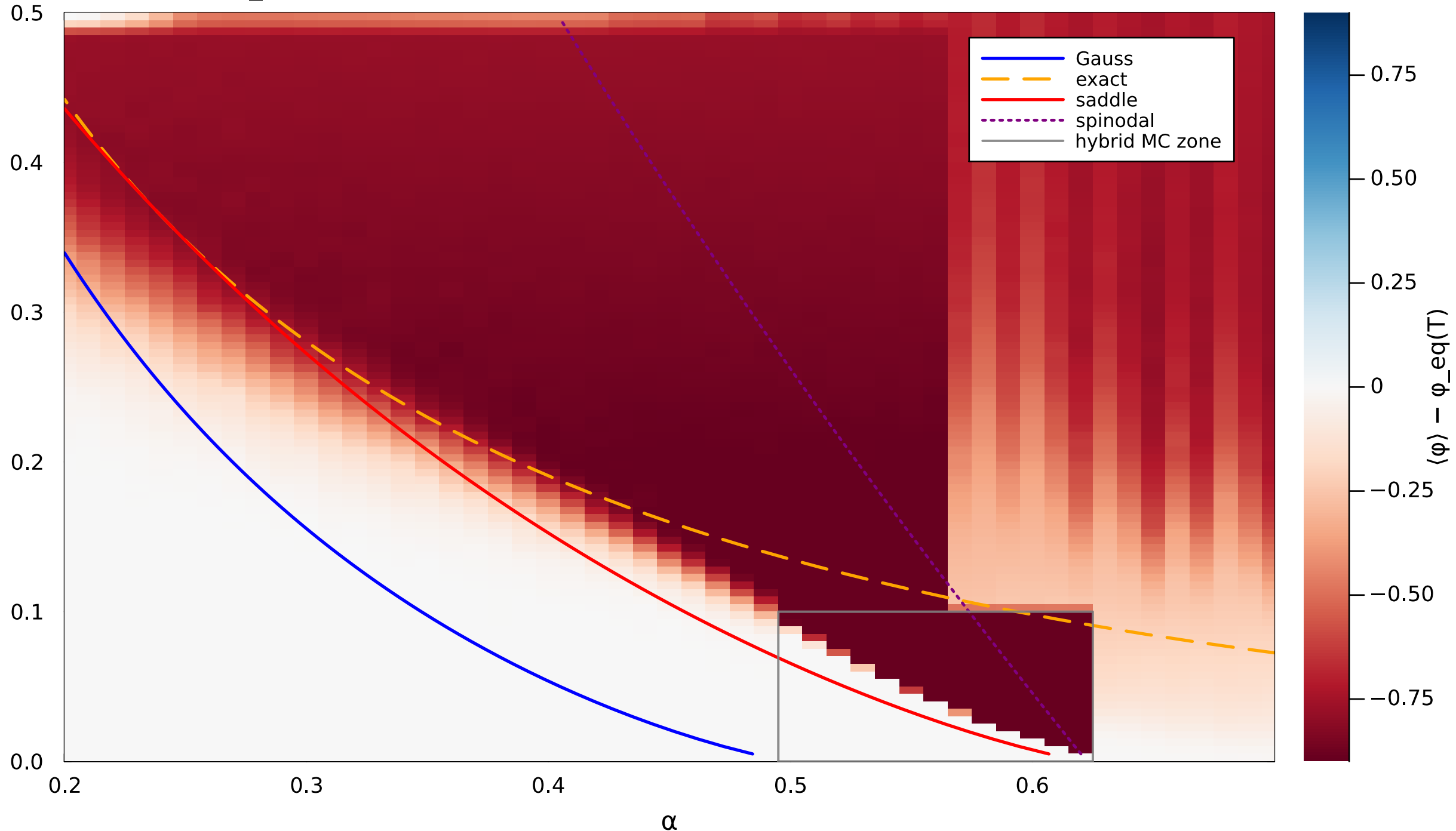
\langle \phi \rangle - \phi_{\text{eq}}(T) , hybrid MC N=100 (priority) \oplus honest N=25 \oplus semismart Nramp
