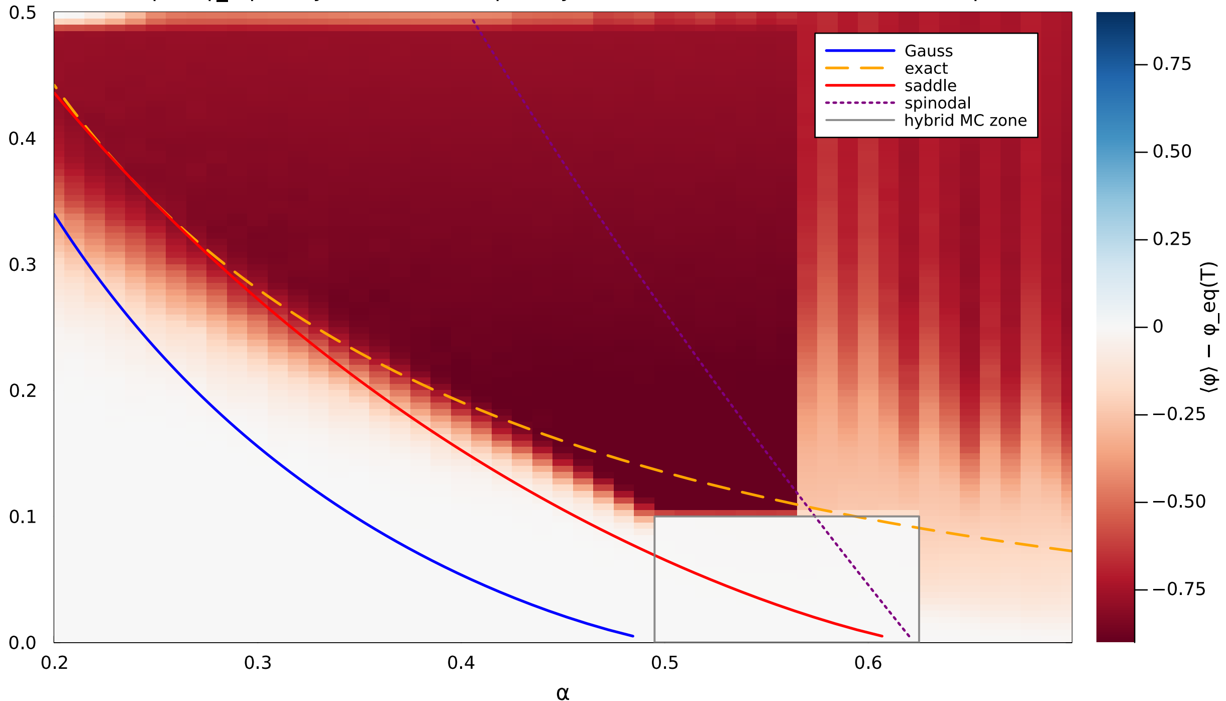
\langle \varphi \rangle - \varphi_{\text{eq}}(T) , hybrid MC N=50 (priority) \oplus honest N=25 \oplus semismart Nramp
