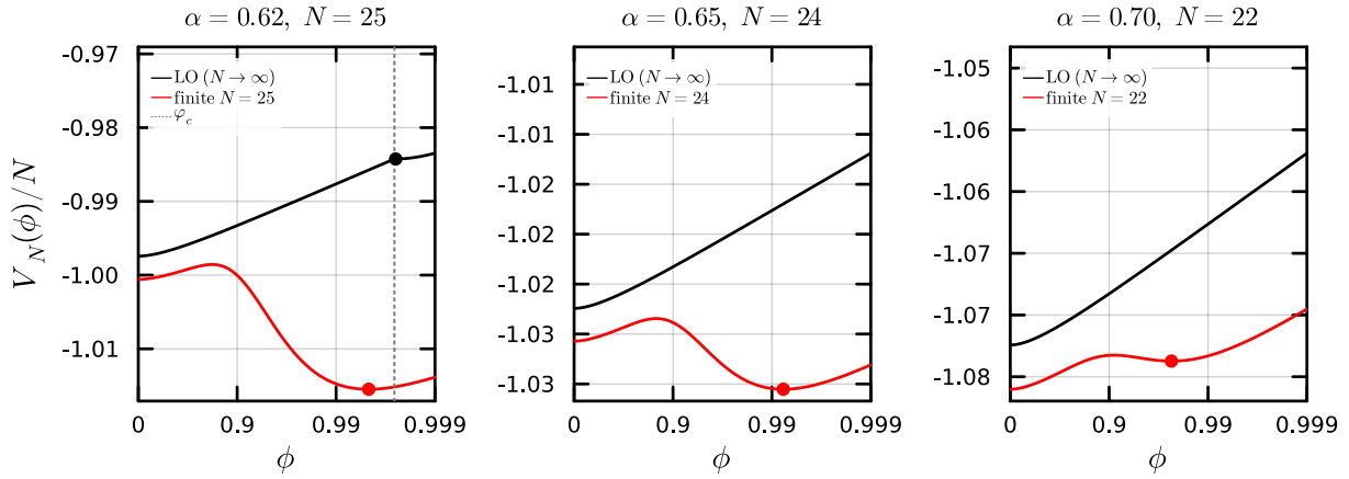
Figure 4: Finite- N effective potential V_N(\phi)/N at \beta = 1 , T = 0.005 , against \phi on a \lg(1 - \phi) axis for three loads above \alpha_c(\beta, 0) = 0.6226 . Black: leading-order landscape -\max(\phi, \varphi_c) - (T/2) \log(1 - \phi^2) . Red: the finite- N form (29) at N(\alpha) for the Cone run at M = 4.4 \times 10^6 . The log-sum smooths the LO corner over width \sim 1/(\beta N) , generating a local minimum near \phi = 1 that the LO curve lacks. Red dots: V_N residual-basin minima. Black dot (left panel only): LO retrieval-basin minimum at \phi = \varphi_{\text{eq}}(T) , present only when \varphi_c < 1 . Grey dotted: LO cusp position \varphi_c , shown only when \varphi_c < 1 .
