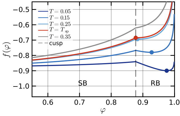
Figure 2: Leading-order free energy density f(\phi) at \alpha = 0.5 , \beta = 1 , for several T . RB: retrieval basin; SB: spurious basin (where the spurious term dominates); cusp at \phi \approx 0.877 (dashed grey). Coloured dots mark the RB minima; they disappear at the spinodal temperature T_{\text{sp}}(\alpha, \beta) \approx 0.262 .
