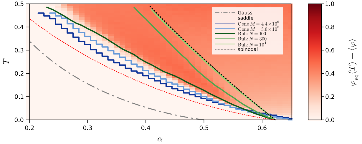
Figure 3: (\alpha, T) stability diagram at \beta = 1 . Heatmap: \varphi_{\text{eq}}(T) - \langle \varphi \rangle from the M = 3.0 \times 10^8 Cone MC run. Blue staircases: Cone retrieval boundary at threshold 0.02 (roughly 5% of chain endpoints escaped) for M = 4.4 \times 10^6 (dark) and M = 3.0 \times 10^8 (light). Green curves: Bulk retrieval boundary at T_{\text{MC}} = 10^5 and N \in \{100, 300, 10^4\} , dark to light with N . The light-green N = 10^4 curve sits on the spinodal across most of the \alpha range; the spinodal is drawn last to make this coincidence visible. Reference curves: saddle boundary \alpha_c^{\text{sd}}(\beta, T) (24) (red dotted), spinodal T_{\text{sp}} (22) (black dotted), Gaussian baseline \alpha_c^{\text{G}}(T) (grey dash-dotted).
