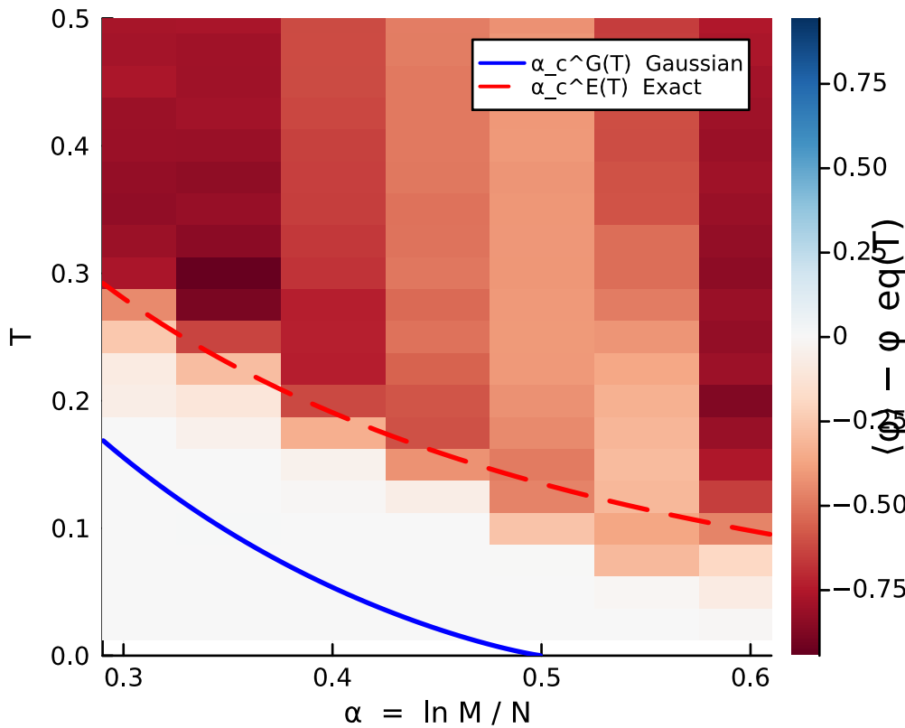
Smart-MC LSE v20 (CPU) N=25 K=10 4 sampled C
