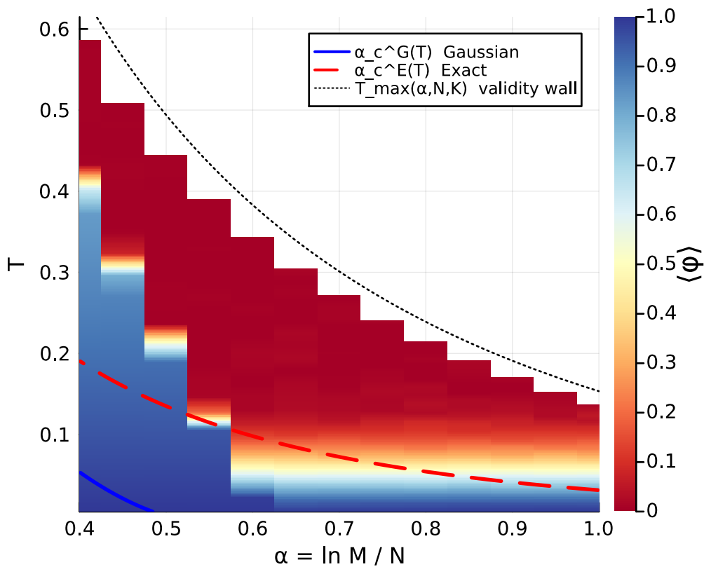
Smart-MC LSE v19 (dynamic) N=500 K=10000
